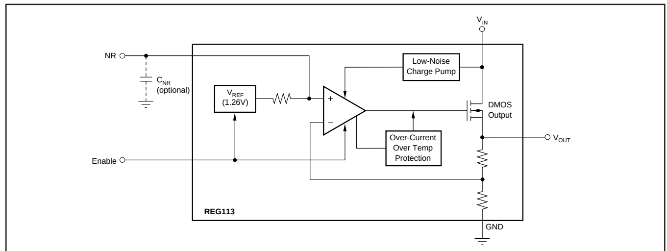
FIGURE 3. Block Diagram.
