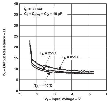
图 7-8. Output Resistance vs Input Voltage
