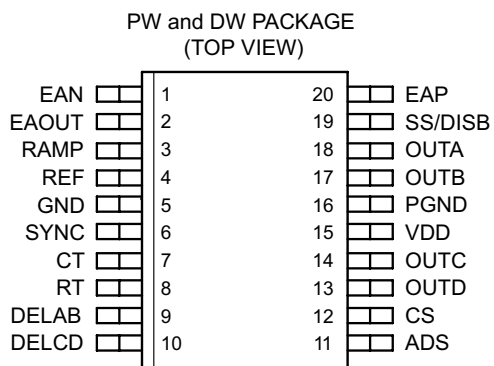
PW AND DW PACKAGE DRAWINGS (TOP VIEW)
