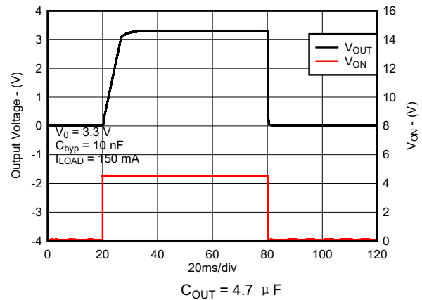
图 8-24. Turn-On Time for New Chip
