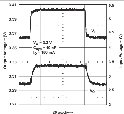
图 8-11. Line Transient Response for Legacy Chip
