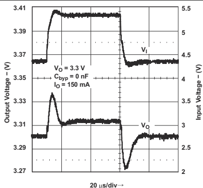
图 8-9. Line Transient Response for Legacy Chip
