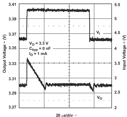
图 8-13. Line Transient Response for Legacy Chip
