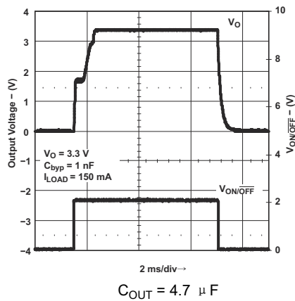
图 8-21. Turn-On Time for Legacy Chip
