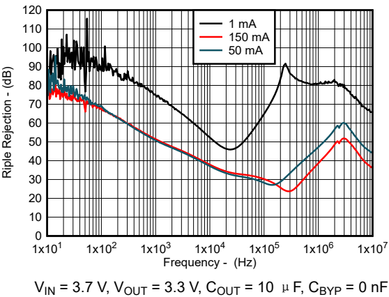
图 6-21. Ripple Rejection vs Frequency for New Chip
