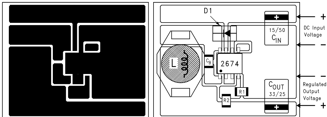
图 9-14. Typical Surface-Mount PCB Layout, Fixed Output (4x Size)
