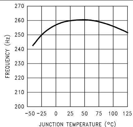
图 7-10. Switching Frequency
