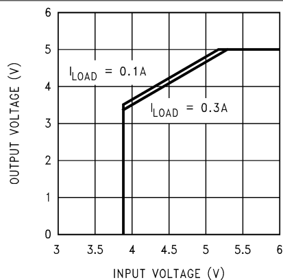
图 7-14. Dropout Voltage, 5-V Version
