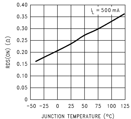
图 7-4. Drain-to-Source Resistance
