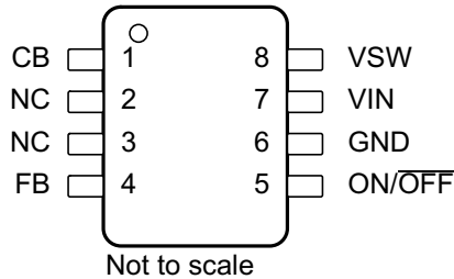
图 6-1. D or P Package 8-Pin SOIC or PDIP Top View
