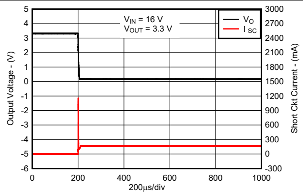
图 6-22. Short-Circuit Current vs Time for New Chip
