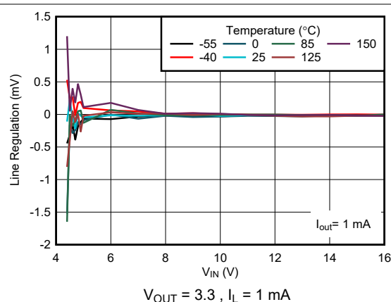
图 5-10. Line Regulation versus V_{IN} & Temperature (New Chip)
