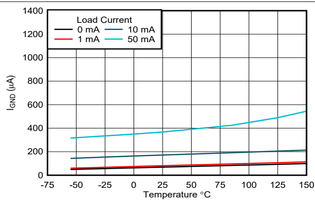
图 5-16. Ground Pin Current ( I_{GND} ) versus Temperature (New Chip)
