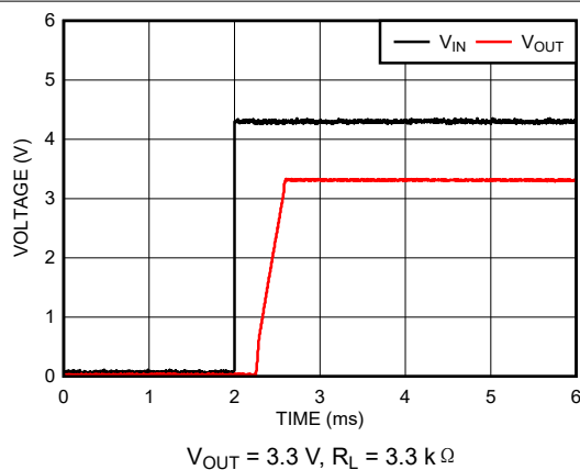
图 7-17. Turn-on Waveform (New Chip)
