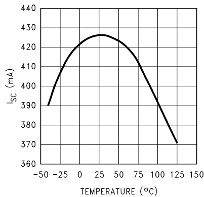
图 5-35. Instantaneous Short Circuit Current versus Temperature (Legacy Chip)
