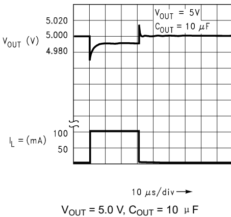
图 5-29. Load Transient Response (Legacy Chip)
