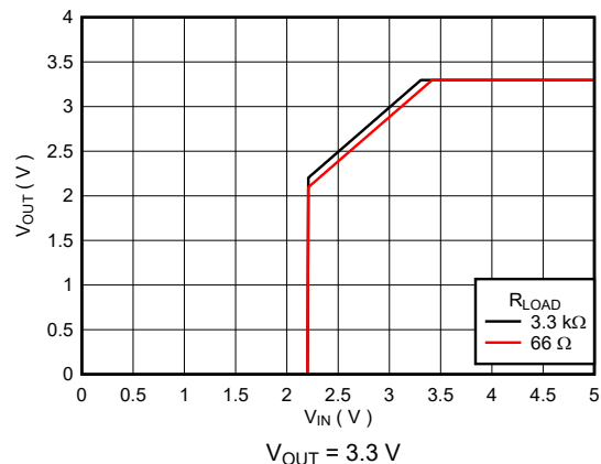
图 5-8. Output Voltage versus V_{IN} (New Chip)
