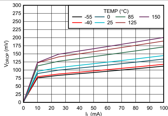
图 5-14. Dropout Voltage ( V_{DO} ) versus Load Current (New Chip)
