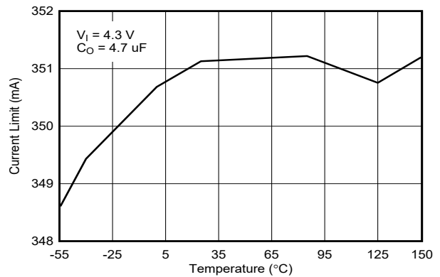
图 5-36. Instantaneous Short Circuit Current versus Temperature (New Chip)
