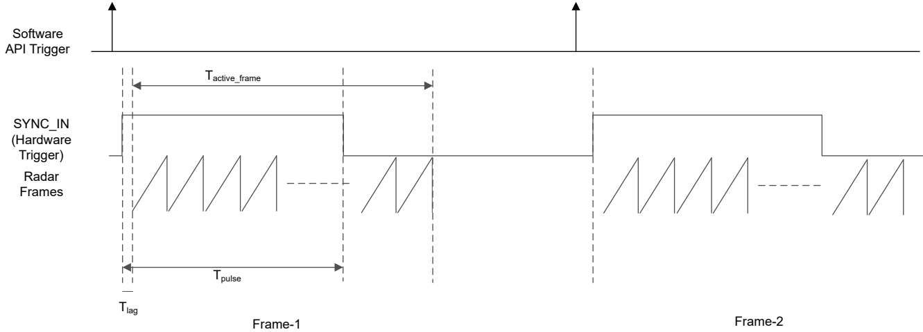
图 8-7. Sync In Hardware Trigger
