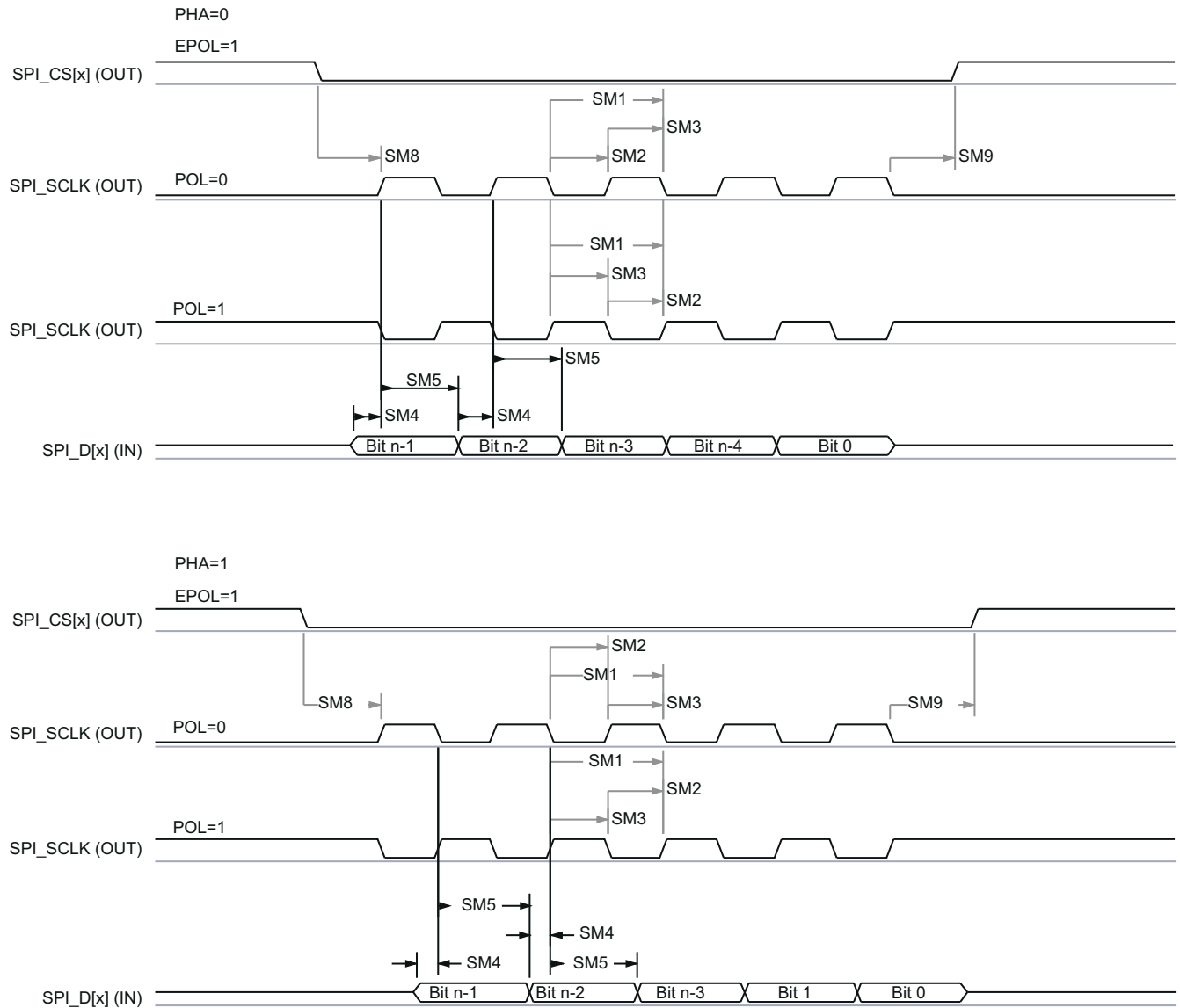
图 7-9. SPI Timing -Controller Mode Receive
