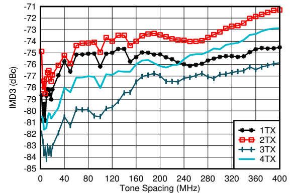
图 4-22. TX IMD3 vs Tone Spacing and Channel at 0.85GHz
