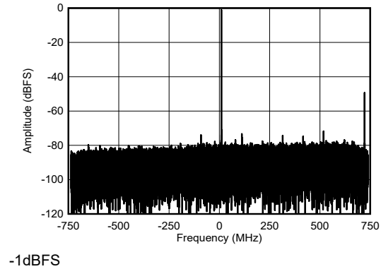
图 4-466. RX Single Tone Output FFT at 9.61 GHz
