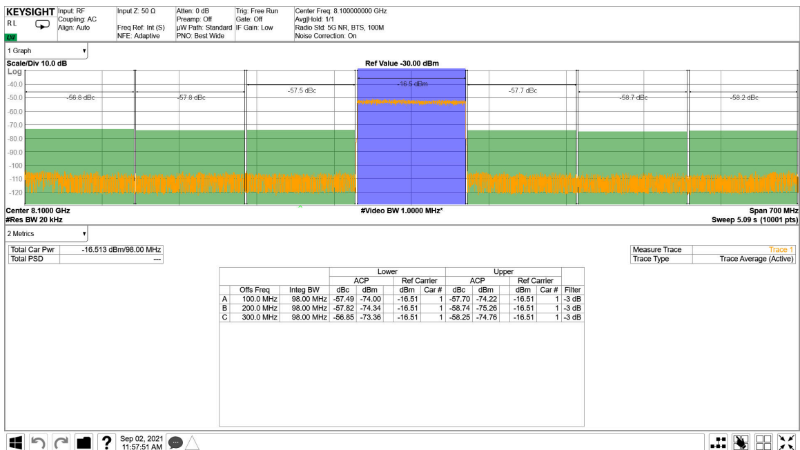
图 4-229. TX 100MHz NR Output Spectrum at 8.1GHz
