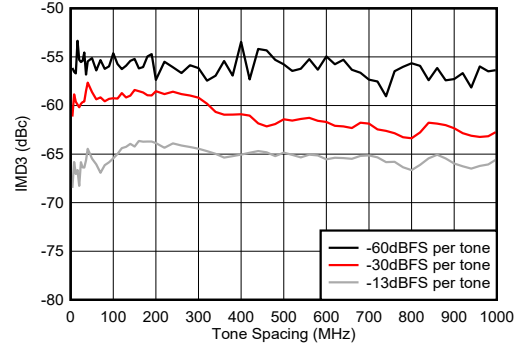
图 4-258. TX IMD3 vs Tone Spacing at 9.61GHz
