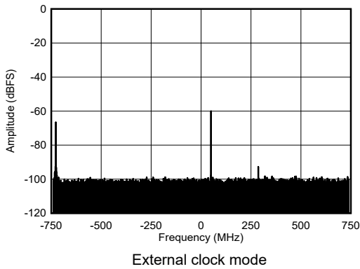
图 4-444. RX Single Tone Output FFT at 8.1GHz, -60 dBFS
