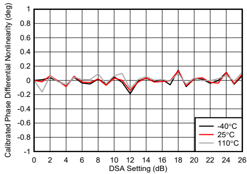
图 4-249. TX DSA Calibrated Phase Integrated Nonlinearity
