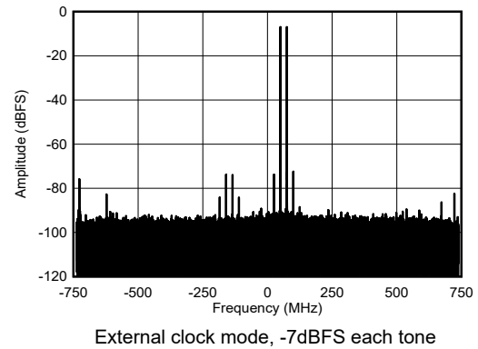
图 4-445. RX Dual Tone Output FFT at 8.1GHz
