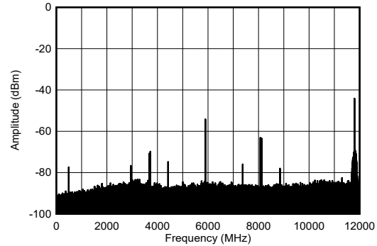
图 4-215. TX Dual Tone Output Spectrum at 8.1GHz
