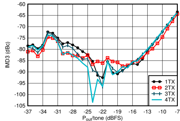
图 4-28. TX IMD3 vs Digital Level at 0.85GHz
