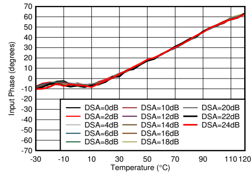
图 4-367. RX Input Phase vs Temperature at 3.6GHz
