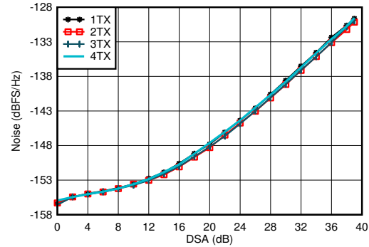
图 4-168. TX Output Noise vs Channel and Attenuation at 2.6GHz
