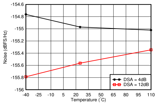
图 4-328. RX Noise Spectral Density vs Temperature at 1.75GHz
