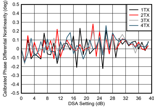
图 4-196. TX DSA Calibrated Phase Differential Nonlinearity at 8.1GHz
