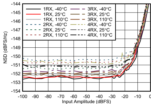
图 4-459. RX NSD vs Digital Amplitude at 9.6GHz
