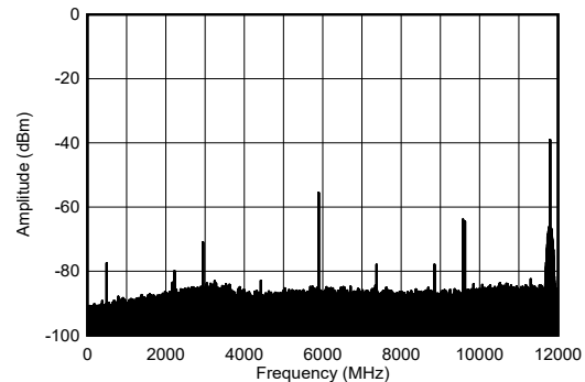
图 4-276. TX 2-Tone Spectrum at 9.61GHz and -30dBFS Each (wideband)
