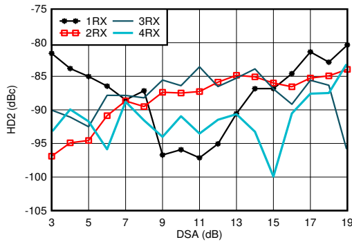
图 4-334. RX HD2 vs DSA Setting and Channel at 1.9 GHz
