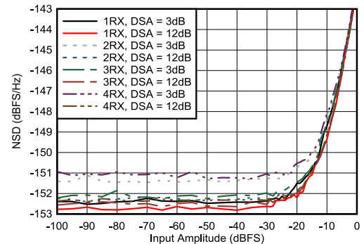
图 4-460. RX NSD vs Digital Amplitude at 9.6GHz
