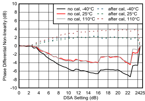
图 4-428. RX Phase Differential Nonlinearity at 8.1GHz
