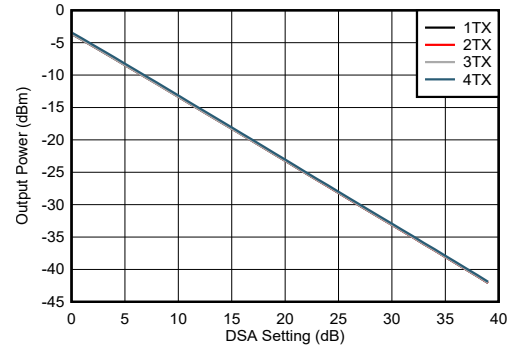
图 4-185. TX Output Power vs DSA Setting at 8.1GHz
