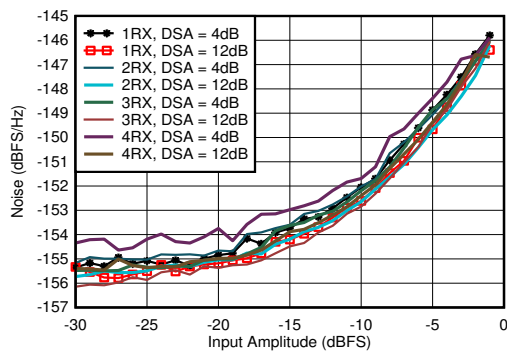
图 4-407. RX Noise Spectral Density vs Input Amplitude and Channel at 4.9GHz
