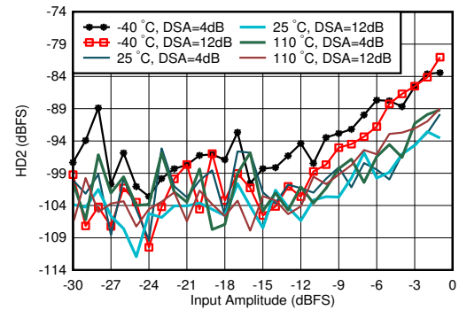
图 4-335. RX HD2 vs DSA Setting and Temperature at 1.9 GHz
