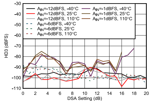
图 4-439. RX HD3 vs DSA Setting at 8.1GHz
