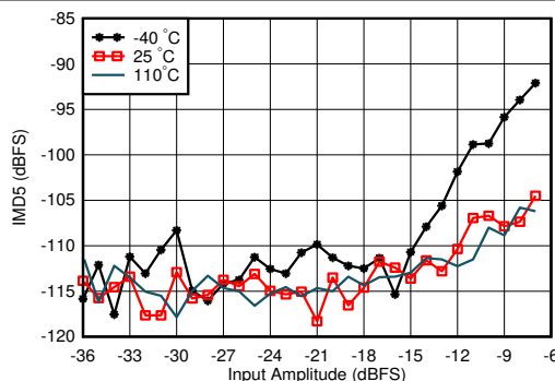
图 4-304. RX IMD5 vs Input Level and Temperature at 0.8GHz
