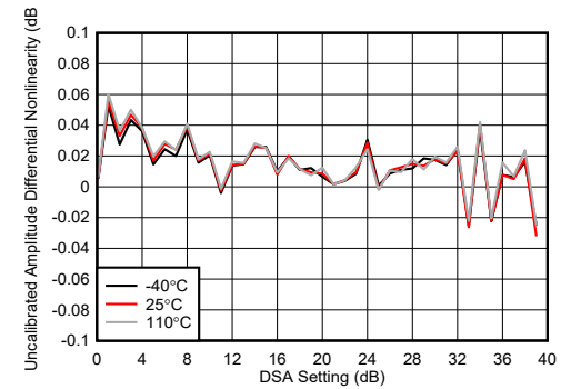
图 4-189. TX DSA Uncalibrated Amplitude Differential Nonlinearity at 8.1GHz
