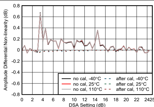
图 4-425. RX Amplitude Differential Nonlinearity at 8.11GHz
