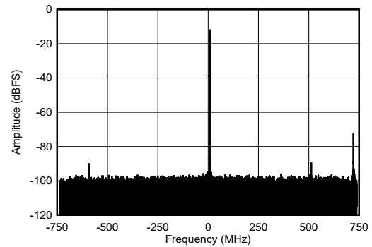
图 4-468. RX Single Tone Output FFT at 9.61GHz
