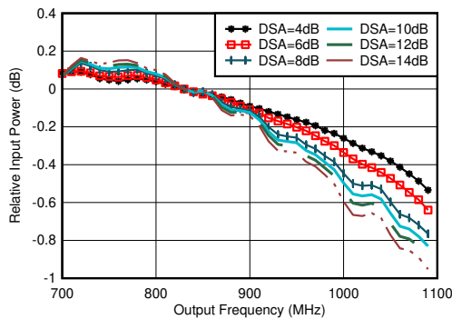
图 4-285. RX In-Band Gain Flatness for Channel 1RX, f_{\text{IN}} = 830\text{MHz}
