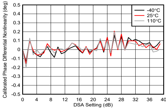
图 4-198. TX DSA Calibrated Phase Differential Nonlinearity at 8.1GHz
