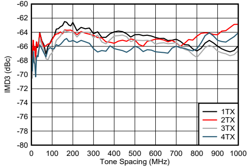
图 4-257. TX IMD3 vs Tone Spacing at 9.61GHz
