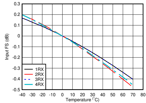
图 4-317. RX Input Fullscale vs Temperature and Channel at 1.75GHz
