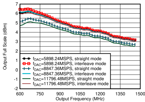
图 4-1. TX Output Fullscale vs Output Frequency
