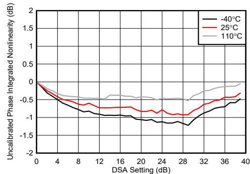
图 4-201. TX DSA Uncalibrated Phase Integrated Nonlinearity at 8.1GHz
