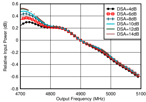
图 4-393. RX Inband Gain Flatness, f_{\text{IN}} = 4900\text{MHz}
