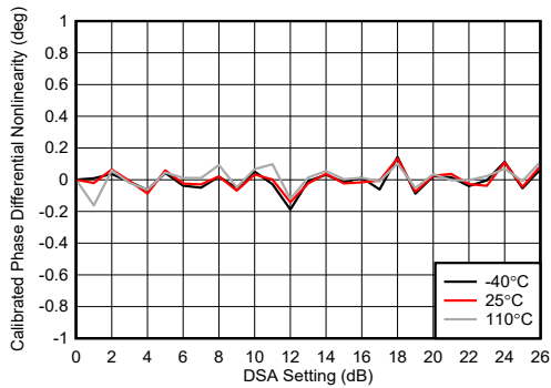
图 4-247. TX DSA Calibrated Phase Differential Nonlinearity
