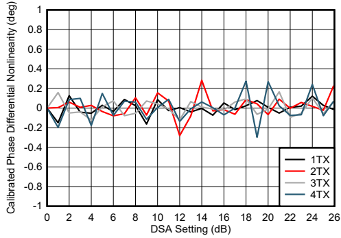
图 4-245. TX DSA Calibrated Phase Differential Nonlinearity
