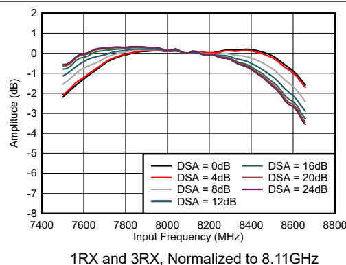
图 4-423. RX Amplitude vs Frequency and DSA Setting
