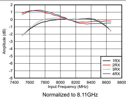
图 4-422. RX Amplitude vs Frequency and Channel
