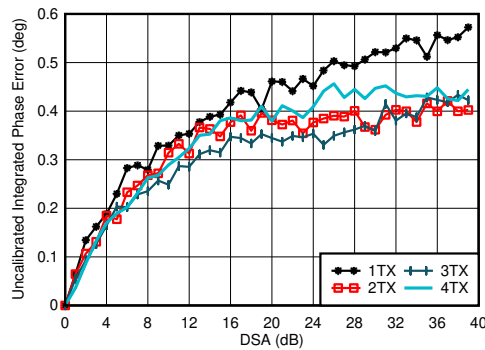
图 4-126. TX Uncalibrated Integrated Phase Error vs DSA Setting and Channel at 3.5GHz
