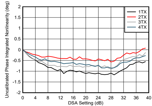
图 4-199. TX DSA Uncalibrated Phase Integrated Nonlinearity at 8.1GHz
