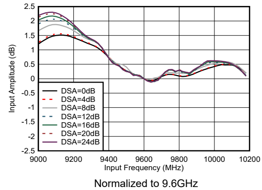
图 4-450. RX Input Amplitude vs Frequency at 9.6GHz
