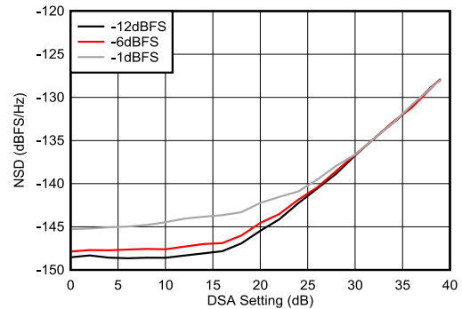
图 4-262. TX NSD vs DSA Setting at 9.61GHz
