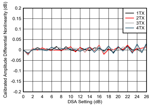
图 4-237. TX DSA Calibrated Amplitude Differential Nonlinearity
