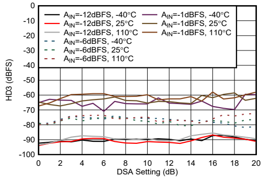
图 4-465. RX HD3 vs DSA Setting at 9.6GHz
