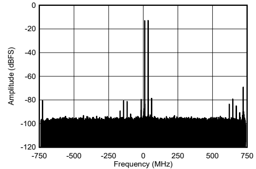
图 4-470. RX Single Tone Output FFT at 9.61GHz
