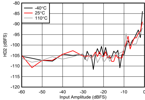
图 4-436. RX HD2 vs Digital Amplitude at 8.1GHz
