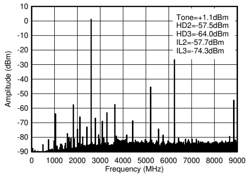
图 4-114. TX Single Tone ( - 12dBFS) Output Spectrum at 2.6GHz ( 0-f_{\text{DAC}} )
