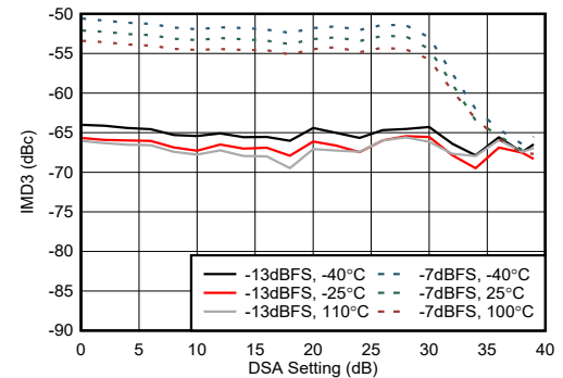
图 4-254. TX IMD3 vs DSA Setting at 9.61GHz
