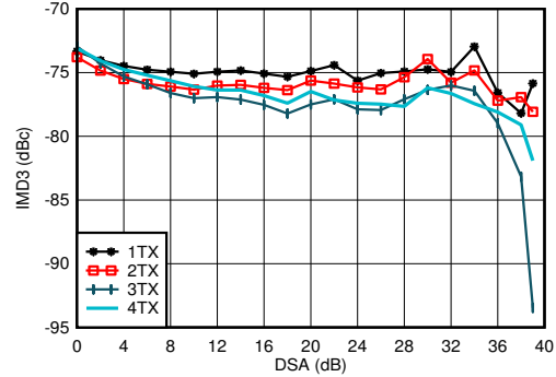
图 4-97. TX IMD3 vs DSA Setting at 2.6GHz
