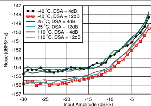
图 4-298. RX Noise Spectral Density vs Input Amplitude and Temperature at 0.8GHz
