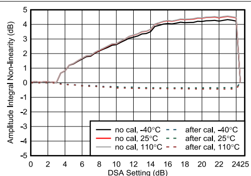
图 4-426. RX Amplitude Integrated Nonlinearity at 8.11GHz
