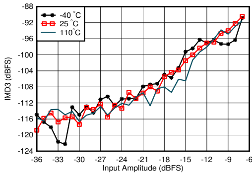
图 4-332. RX IMD3 vs Input Level and Temperature at 1.75GHz
