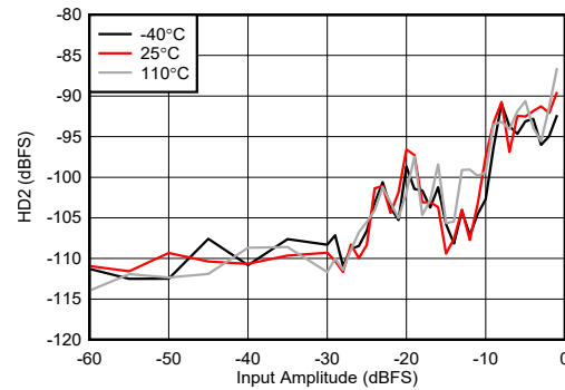
图 4-462. RX HD2 vs Digital Level at 9.6GHz
