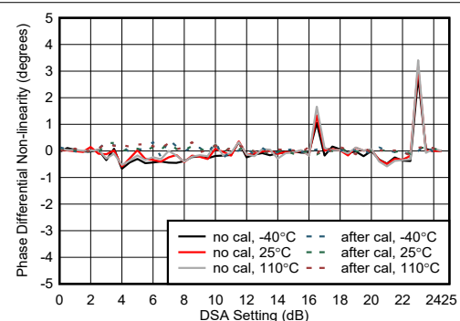
图 4-427. RX Phase Differential Nonlinearity at 8.11GHz
