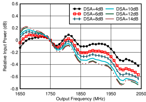
图 4-316. RX In-Band Gain Flatness, f_{\text{IN}} = 1750\text{MHz}
