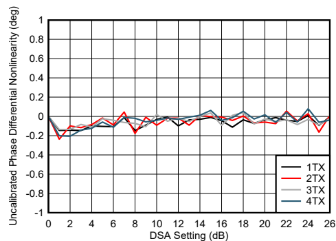
图 4-244. TX DSA Uncalibrated Phase Differential Nonlinearity
