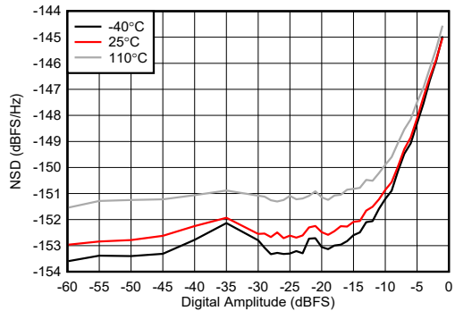
图 4-261. TX NSD vs Digital Amplitude at 9.61GHz
