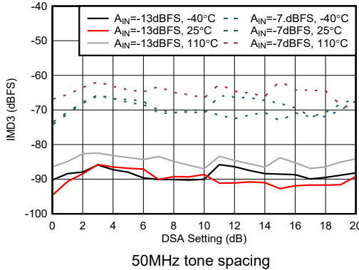
图 4-457. RX IMD3 vs DSA Setting at 9.6GHz
