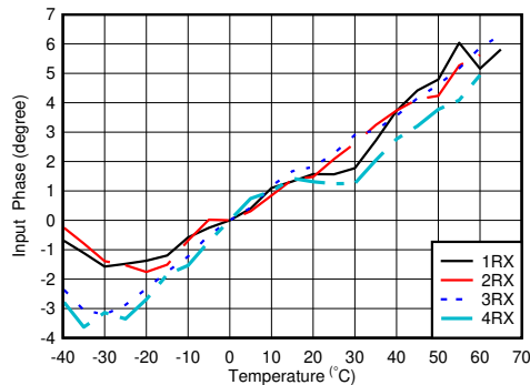
图 4-287. RX Input Phase vs Temperature and DSA at f_{\text{OUT}} = 0.8\text{GHz}
