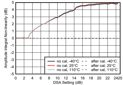
图 4-452. RX Amplitude Integrated Non-linearity at 9.6GHz
