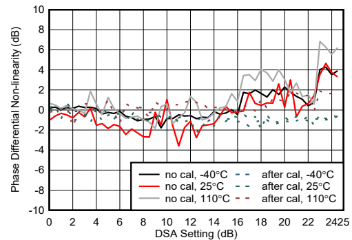
图 4-454. RX Phase Integrated Non-linearity at 9.6GHz
