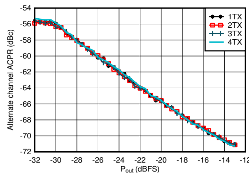
图 4-176. TX 20MHz LTE alt-ACPR vs Digital Level at 4.9GHz
