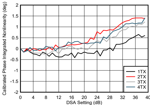
图 4-200. TX DSA Calibrated Phase Integrated Nonlinearity at 8.1GHz
