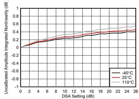
图 4-242. TX DSA Uncalibrated Amplitude Integrated Nonlinearity
