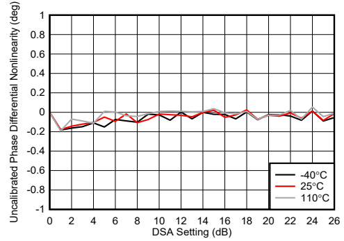
图 4-246. TX DSA Uncalibrated Phase Differential Nonlinearity
