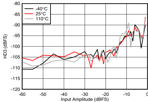
图 4-438. RX HD3 vs Digital Amplitude at 8.1GHz
