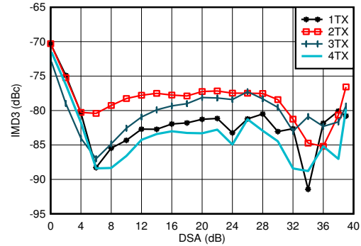
图 4-63. TX IMD3 vs DSA Setting at 1.8GHz
