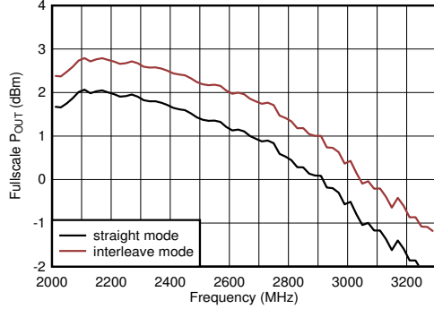
图 4-78. TX Full Scale vs RF Frequency at 11796.48MSPS
