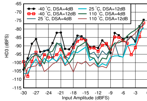
图 4-341. RX HD3 vs Input Level and Temperature at 1.9GHz
