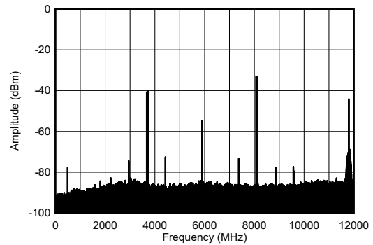
图 4-211. TX Dual Tone Output Spectrum at 8.11GHz
