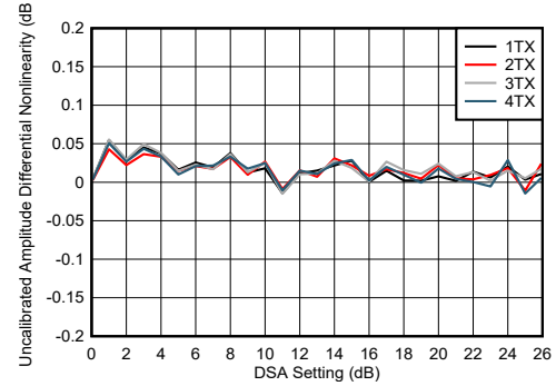
图 4-236. TX DSA Uncalibrated Amplitude Differential Nonlinearity
