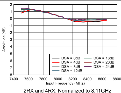
图 4-424. RX Amplitude vs Frequency and DSA Setting
