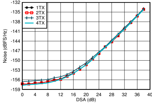
图 4-96. TX Output Noise vs Channel and Attenuation at 2.6GHz
