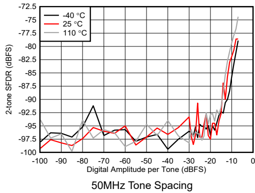
图 4-440. RX 2-tone SFDR vs Digital Amplitude at 8.1GHz
