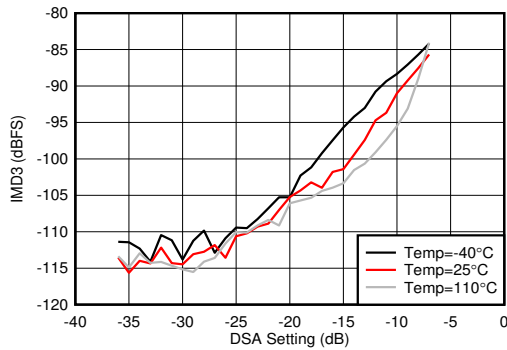
图 4-378. RX IMD3 vs Input Level and Temperature at 3.6GHz
