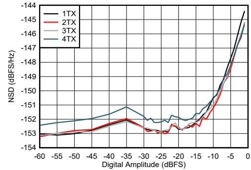
图 4-260. TX NSD vs Digital Amplitude at 9.61GHz
