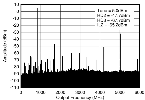
图 4-43. TX Single Tone ( - 1dBFS) Output Spectrum at 0.85GHz (0- f_{\text{DAC}} )
