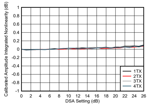
图 4-241. TX DSA Calibrated Amplitude Integrated Nonlinearity
