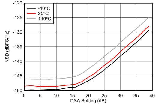
图 4-264. TX NSD vs DSA Setting at 9.61GHz
