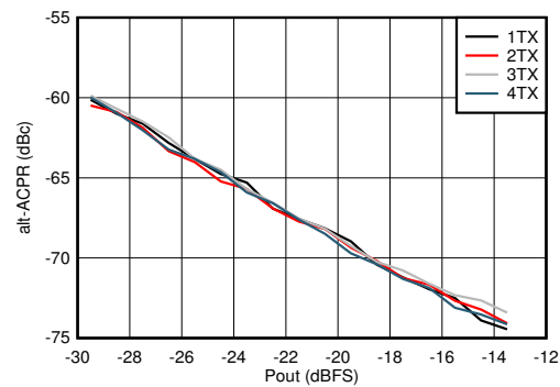
图 4-105. TX 20-MHz LTE alt-ACPR vs Digital Level at 2.6GHz
