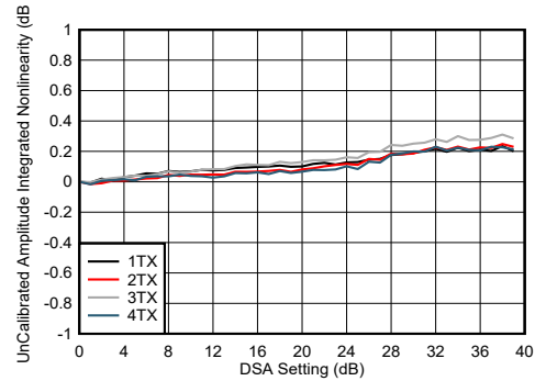
图 4-191. TX DSA Uncalibrated Amplitude Integrated Nonlinearity at 8.1GHz
