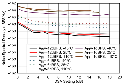
图 4-434. RX NSD vs DSA Setting at 8.1GHz
