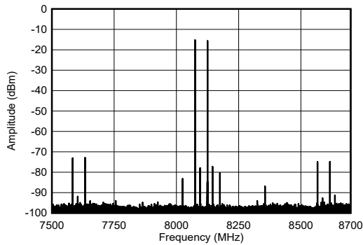
图 4-210. TX Dual Tone Output Spectrum at 8.11GHz
