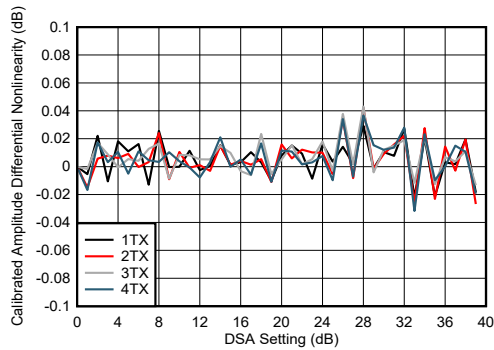
图 4-188. TX DSA Calibrated Amplitude Differential Nonlinearity at 8.1GHz
