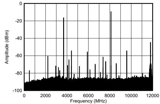
图 4-203. TX Single Tone Output Spectrum at 8.1GHz
