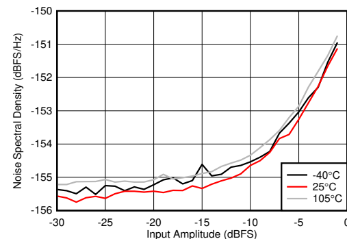
图 4-351. RX Noise Spectral Density vs Input Amplitude and Temperature at 2.6GHz
