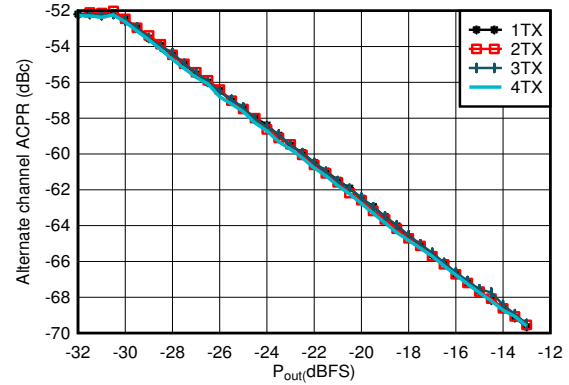
图 4-34. TX 20MHz LTE alt-ACPR vs Digital Level at 0.85GHz
