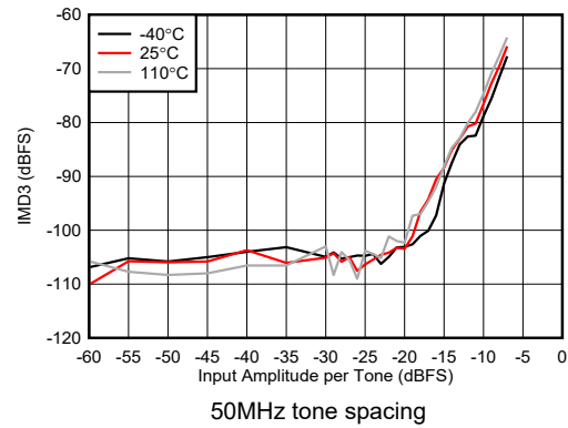
图 4-429. RX IMD3 vs Input Amplitude at 8.1GHz
