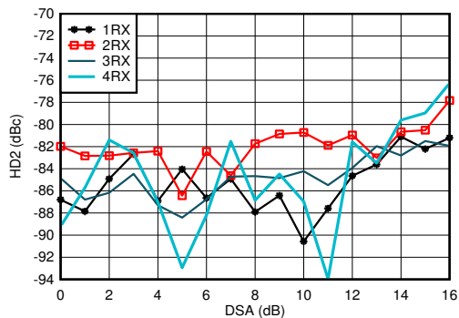
图 4-411. RX HD2 vs DSA Setting and Channel at 4.9GHz
