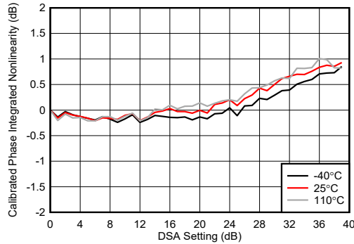
图 4-202. TX DSA Calibrated Phase Integrated Nonlinearity at 8.1GHz
