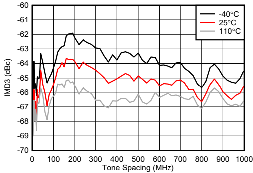
图 4-259. TX IMD3 vs Tone Spacing at 9.61GHz
