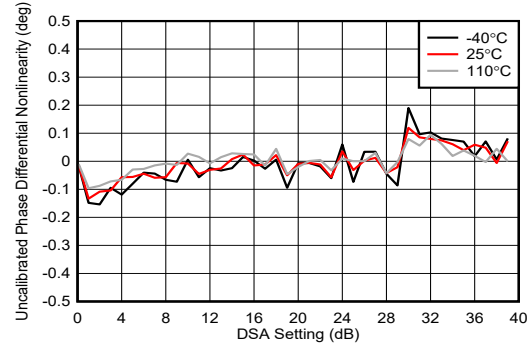
图 4-197. TX DSA Uncalibrated Phase Differential Nonlinearity at 8.1GHz
