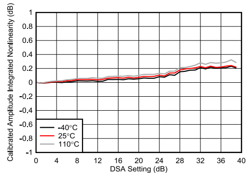
图 4-194. TX DSA Calibrated Amplitude Integrated Nonlinearity at 8.1GHz
