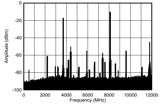
图 4-209. TX Dual Tone Output Spectrum at 8.11GHz
