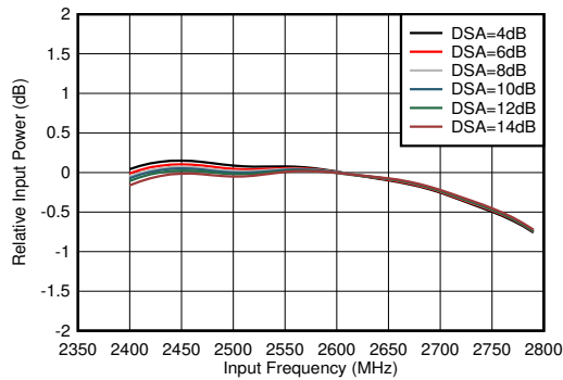
图 4-346. RX Inband Gain Flatness, f_{\text{IN}} = 2600\text{MHz}
