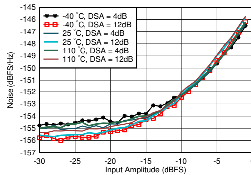
图 4-329. RX Noise Spectral Density vs Input Amplitude and Temperature at 1.75GHz
