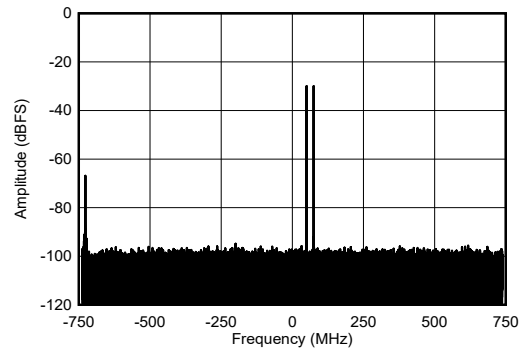
图 4-447. RX Dual Tone Output FFT at 8.1GHz
