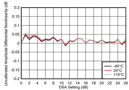
图 4-238. TX DSA Uncalibrated Amplitude Differential Nonlinearity
