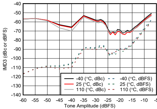
图 4-253. TX IMD3 vs Digital Amplitude at 9.61GHz
