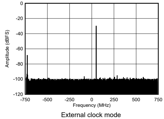
图 4-443. RX Single Tone Output FFT at 8.1GHz, -30 dBFS
