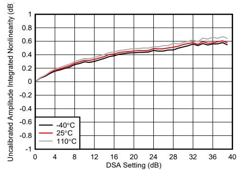
图 4-193. TX DSA Uncalibrated Amplitude Integrated Nonlinearity at 8.1GHz
