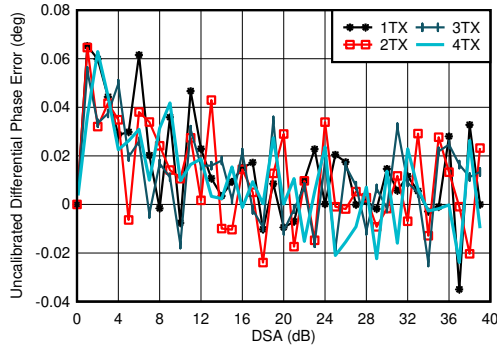
图 4-124. TX Uncalibrated Differential Phase Error vs DSA Setting and Channel at 3.5GHz
