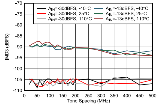
图 4-431. RX IMD3 vs Tone Spacing at 8.1GHz
