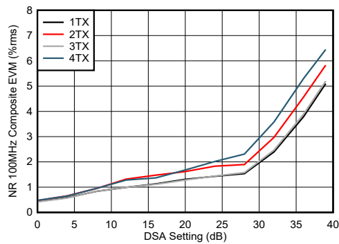
图 4-228. TX NR100MHz EVM vs DSA Setting 8.1GHz
