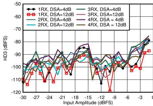
图 4-340. RX HD3 vs Input Level and Channel at 1.9GHz
