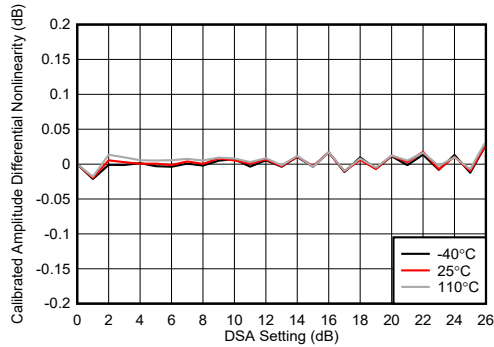
图 4-239. TX DSA Calibrated Amplitude Differential Nonlinearity
