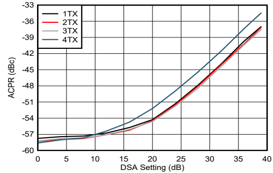
图 4-227. TX NR100MHz alt-ACPR vs DSA Setting 8.1GHz
