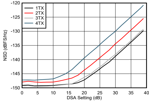
图 4-263. TX NSD vs DSA Setting at 9.61GHz
