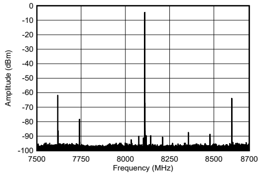
图 4-204. TX Single Tone Output Spectrum at 8.1GHz
