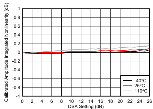
图 4-243. TX DSA Calibrated Amplitude Integrated Nonlinearity
