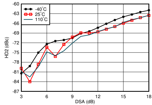
图 4-306. RX HD2 vs DSA Setting and Temperature at 0.8GHz
