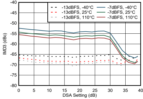
图 4-220. TX IMD3 vs DSA Setting at 8.11GHz
