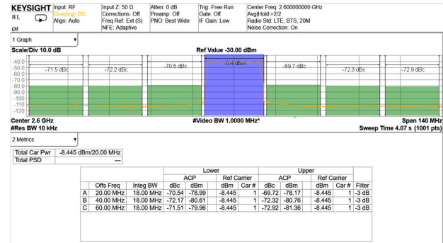
图 4-103. TX 20-MHz LTE Output Spectrum at 2.6GHz (Band 41)
