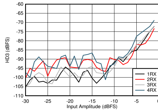
图 4-385. RX HD3 vs Input Level and Channel at 3.6GHz
