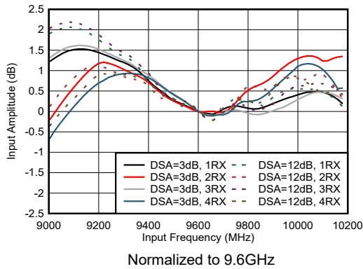
图 4-449. RX Input Amplitude vs Frequency
