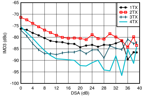
图 4-21. TX IMD3 vs DSA Setting at 0.85GHz
