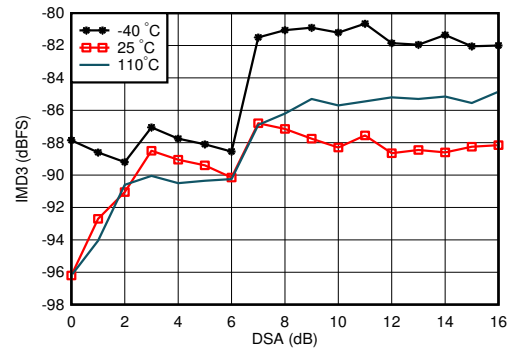
图 4-300. RX IMD3 vs DSA Setting and Temperature at 0.8GHz
