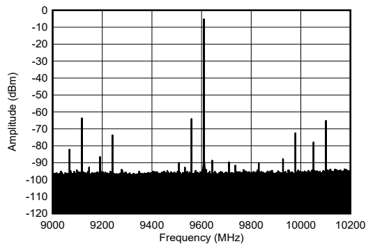
图 4-267. TX Single Tone Spectrum at 9.61GHz and -1dBFS (1.2GHz BW)
