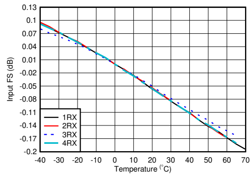
图 4-286. RX Input Fullscale vs Temperature and Channel at 800MHz
