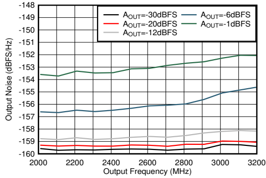
图 4-102. TX Single Tone Output Noise vs Frequency and Amplitude at 2.6GHz
