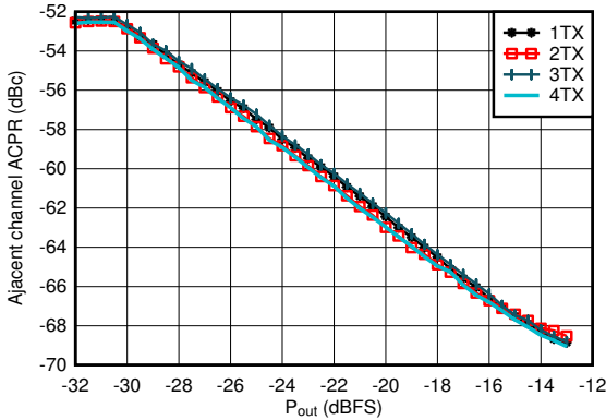
图 4-33. TX 20-MHz LTE ACPR vs Digital Level at 0.85GHz
