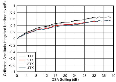
图 4-192. TX DSA Calibrated Amplitude Integrated Nonlinearity at 8.1GHz
