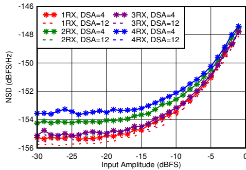
图 4-352. RX Noise Spectral Density vs Input Amplitude and Channel at 2.6GHz
