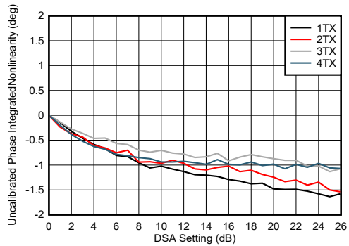
图 4-248. TX DSA Uncalibrated Phase Integrated Nonlinearity
