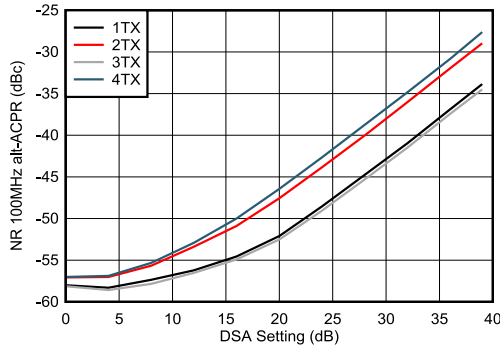
图 4-281. TX NR100MHz ACPR vs DSA Setting at 9.61GHz NR100MHz alt-ACPR vs DSA Setting at 9.61GHz
