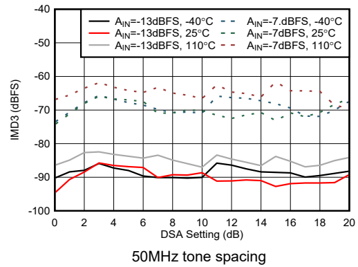
图 4-456. RX IMD3 vs DSA Setting at 9.6GHz
