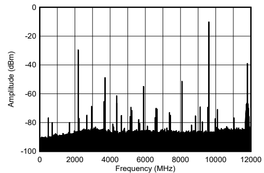
图 4-266. TX Single Tone Spectrum at 9.61GHz and -1dBFS (wideband)
