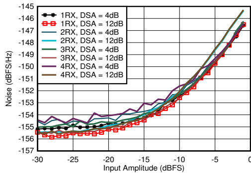
图 4-330. RX Noise Spectral Density vs Input Amplitude and Channel at 1.75GHz
