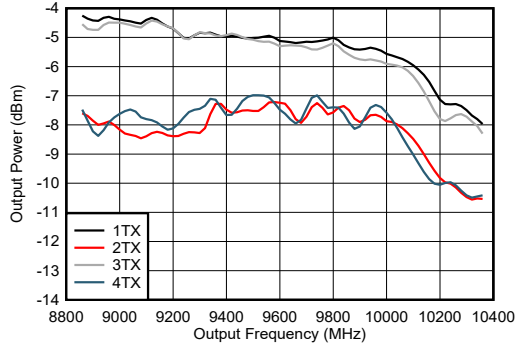
图 4-233. TX Output Power vs Frequency at 9.61GHz
