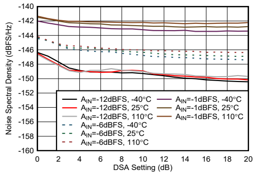
图 4-461. RX NSD vs DSA Setting at 9.6GHz
