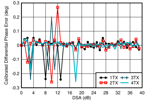
图 4-125. TX Calibrated Differential Phase Error vs DSA Setting and Channel at 3.5GHz
