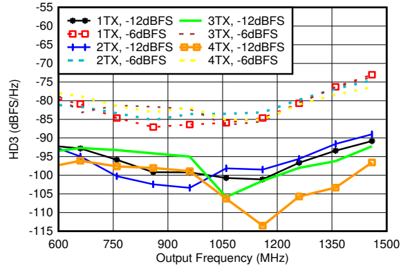
图 4-39. TX HD3 vs Digital Amplitude and Output Frequency at 0.85GHz
