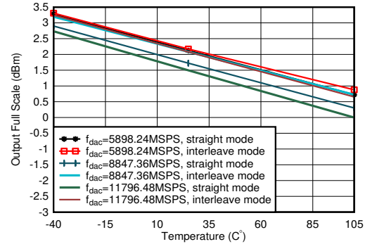
图 4-45. TX Output Power vs Temperature at 1.8GHz
