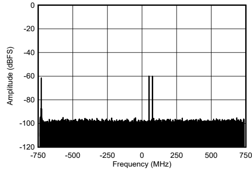
图 4-446. RX Dual Tone Output FFT at 8.1GHz
