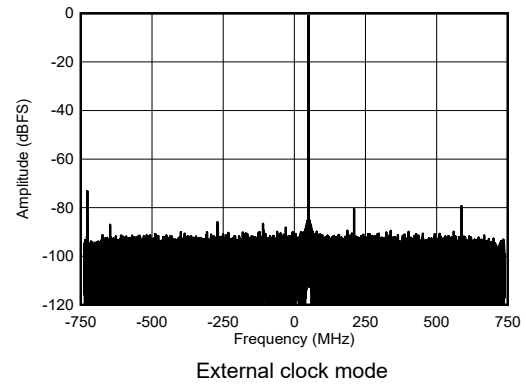
图 4-441. RX Single Tone Output FFT at 8.1GHz, -1dBFS
