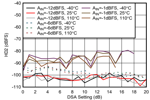
图 4-437. RX HD2 vs DSA Setting at 8.1GHz
