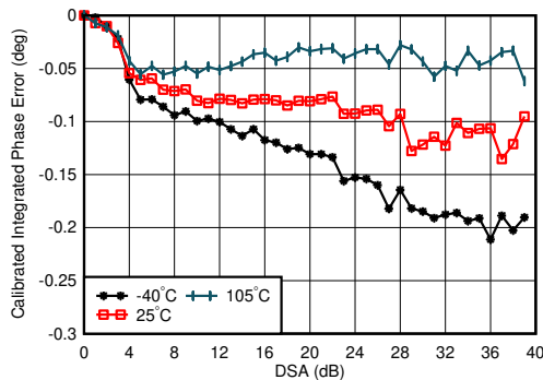
图 4-17. TX Calibrated Differential Phase Error vs DSA Setting and Temperature at 0.85GHz
