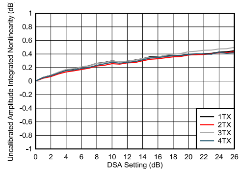
图 4-240. TX DSA Uncalibrated Amplitude Integrated Nonlinearity
