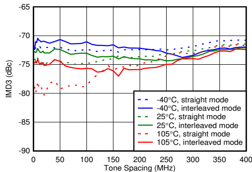
图 4-99. TX IMD3 vs Tone Spacing and Temperature at 2.6GHz
