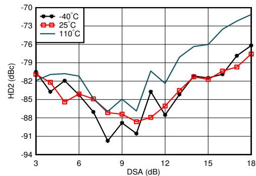
图 4-412. RX HD2 vs DSA and Temperature at 4.9GHz
