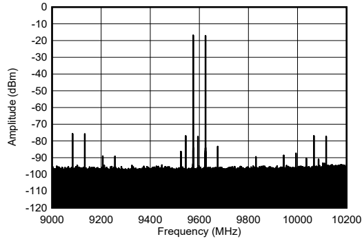
图 4-275. TX 2-Tone Spectrum at 9.61GHz and -13dBFS (1.2GHz BW)
