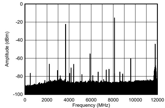
图 4-205. TX Single Tone Output Spectrum at 8.1GHz
