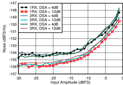
图 4-299. RX Noise Spectral Density vs Input Amplitude and Channel at 0.8GHz
