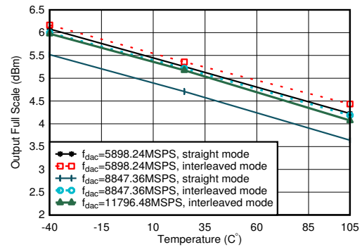
图 4-2. TX Output Fullscale vs Temperature
