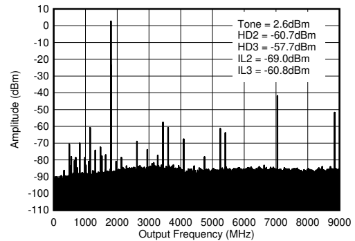
图 4-75. TX Single Tone ( - 12 dBFS) Output Spectrum at 1.8GHz ( 0-f_{DAC} )
