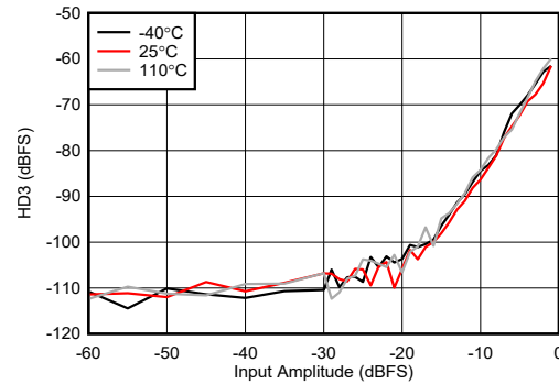
图 4-464. RX HD3 vs Digital Level at 9.6GHz
