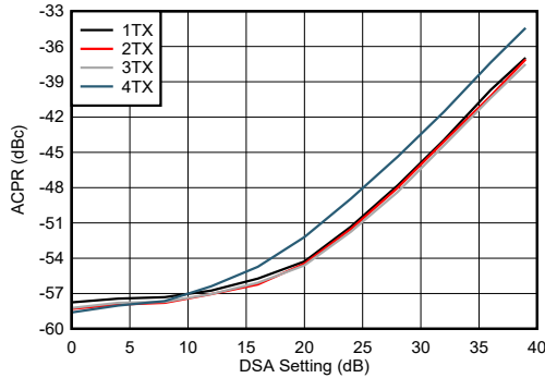
图 4-226. TX NR100MHz ACPR vs DSA Setting 8.1GHz
