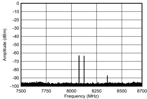
图 4-214. TX Dual Tone Output Spectrum at 8.1GHz
