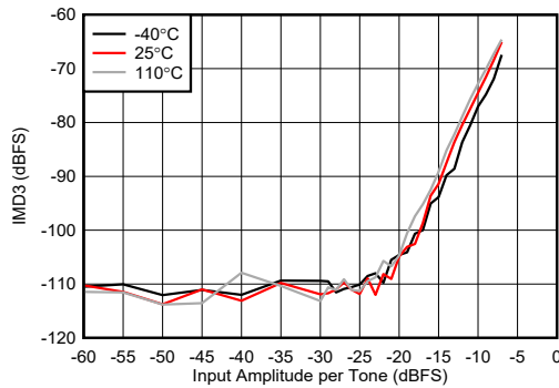
图 4-455. RX IMD3 vs Digital Amplitude at 9.6GHz
