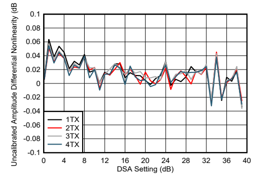
图 4-187. TX DSA Uncalibrated Amplitude Differential Nonlinearity at 8.1GHz
