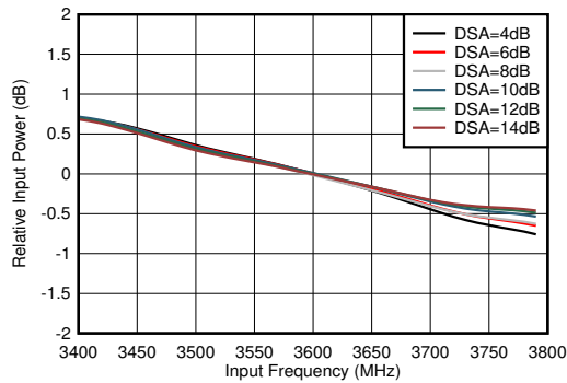
图 4-366. RX In-Band Gain Flatness, f_{\text{IN}} = 3600\text{MHz}
