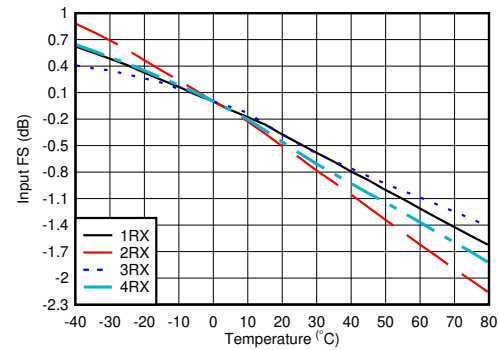
图 4-394. RX Input Fullscale vs Temperature and Channel at 4.9GHz
