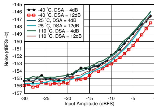
图 4-406. RX Noise Spectral Density vs Input Amplitude and Temperature at 4.9GHz
