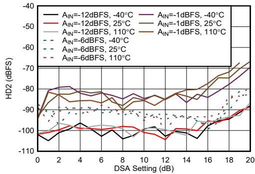
图 4-463. RX HD2 vs DSA Setting at 9.6GHz
