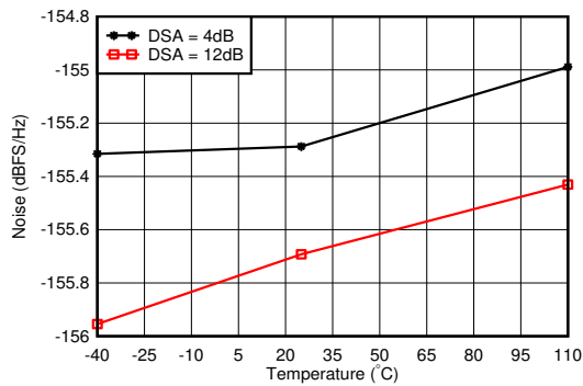
图 4-405. RX Noise Spectral Density vs Temperature at 4.9GHz
