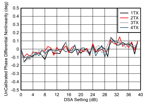
图 4-195. TX DSA Uncalibrated Phase Differential Nonlinearity at 8.1GHz
