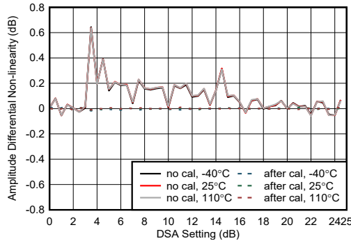
图 4-451. RX Amplitude Differential Non-linearity at 9.6GHz
