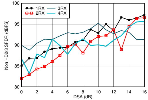
图 4-312. RX Non-HD2/3 vs DSA Setting at 0.8GHz
