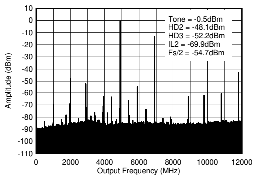
图 4-183. TX Single Tone ( - 1 dBFS) Output Spectrum at 4.9GHz (0- f_{\text{DAC}} )
