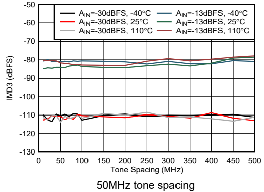
图 4-458. RX IMD3 vs Tone Spacing at 9.6GHz
