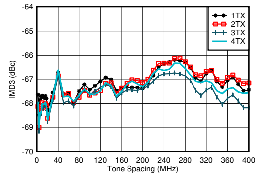
图 4-170. TX IMD3 vs Tone Spacing and Channel at 4.9GHz
