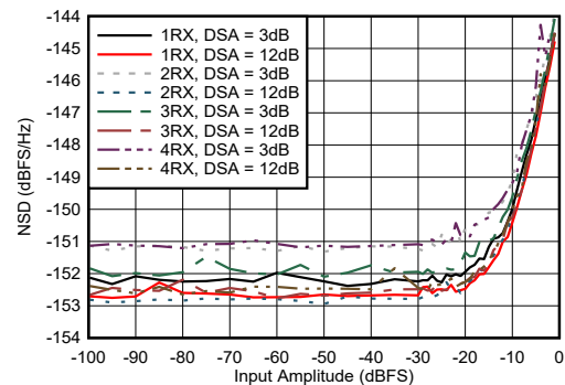
图 4-433. RX NSD vs Digital Amplitude at 8.1GHz
