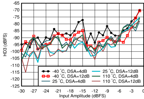
图 4-311. RX HD3 vs Input Level and Temperature at 0.8GHz
