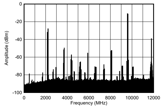
图 4-270. TX Single Tone Spectrum at 9.61GHz and -12dBFS (wideband)
