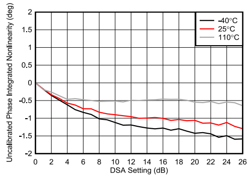
图 4-250. TX DSA Uncalibrated Phase Integrated Nonlinearity
