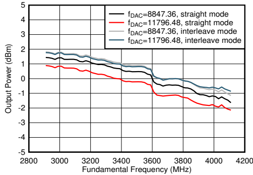
图 4-118. TX Output Power vs Frequency
