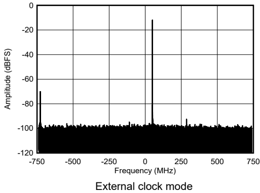
图 4-442. RX Single Tone Output FFT at 8.1GHz, -12dBFS
