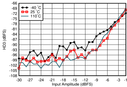
图 4-417. RX HD3 vs Input Level and Temperature at 4.9GHz
