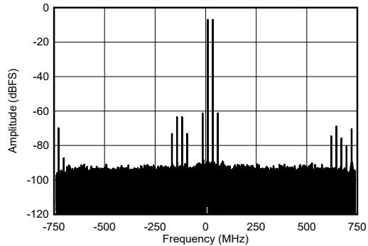
图 4-469. RX Single Tone Output FFT at 9.61GHz
