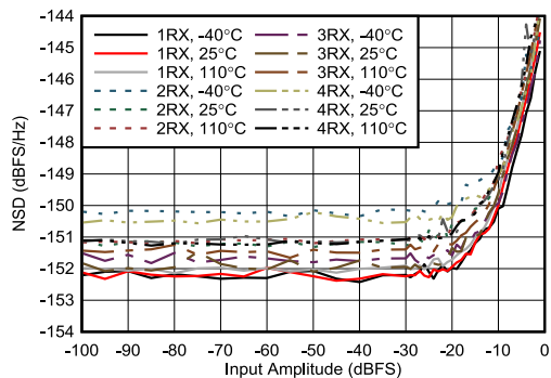
图 4-432. RX NSD vs Digital Amplitude at 8.1GHz
