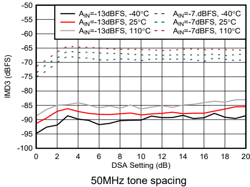
图 4-430. RX IMD3 vs DSA Setting at 8.1GHz
