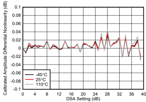
图 4-190. TX DSA Calibrated Amplitude Differential Nonlinearity at 8.1GHz
