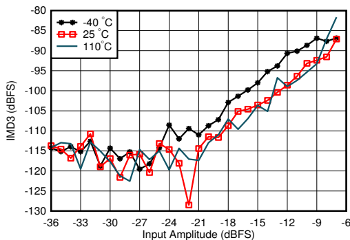
图 4-409. RX IMD3 vs Input Level and Temperature at 4.9GHz
