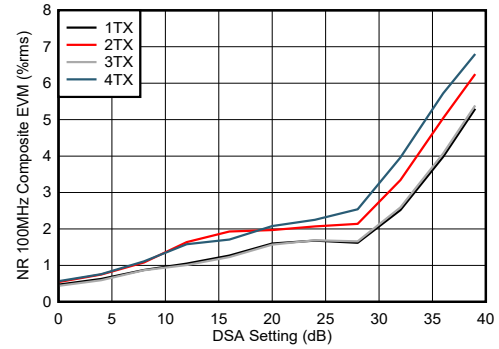
图 4-282. TX NR100MHz EVM vs DSA Setting at 9.61GHz
