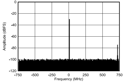
图 4-467. RX Single Tone Output FFT at 9.61GHz
