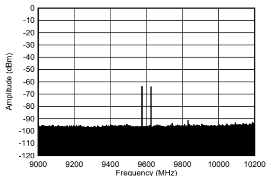
图 4-277. TX 2-Tone Spectrum at 9.61GHz and -30dBFS Each (1.2GHz BW)
