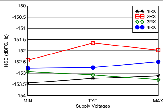
图 4-365. RX Noise Spectral Density vs Supply and Channel at 2.6GHz
