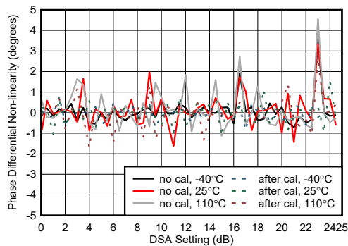
图 4-453. RX Phase Differential Non-linearity at 9.6GHz
