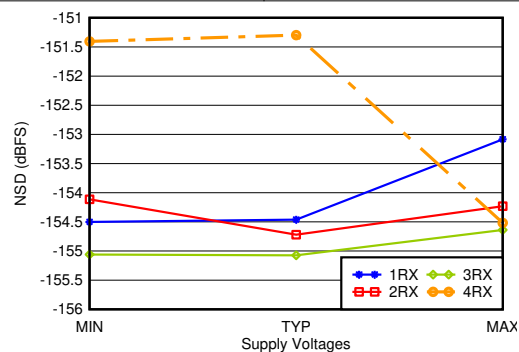
图 4-420. RX IMD3 vs Supply and Channel at 4.9GHz
