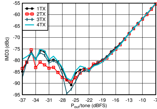
图 4-172. TX IMD3 vs Digital Level at 4.9GHz
