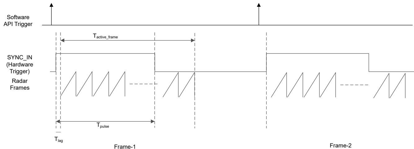
图 7-9. Sync In Hardware Trigger
