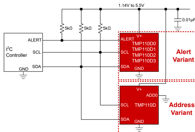
Figure 3-1. Simplified Schematic
