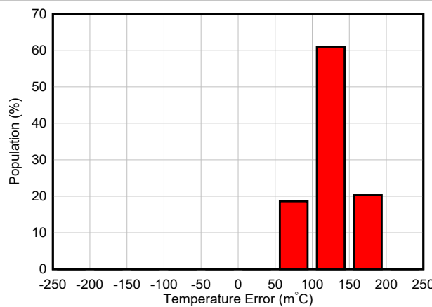
Figure 6-12. Temperature Error at 25°C
