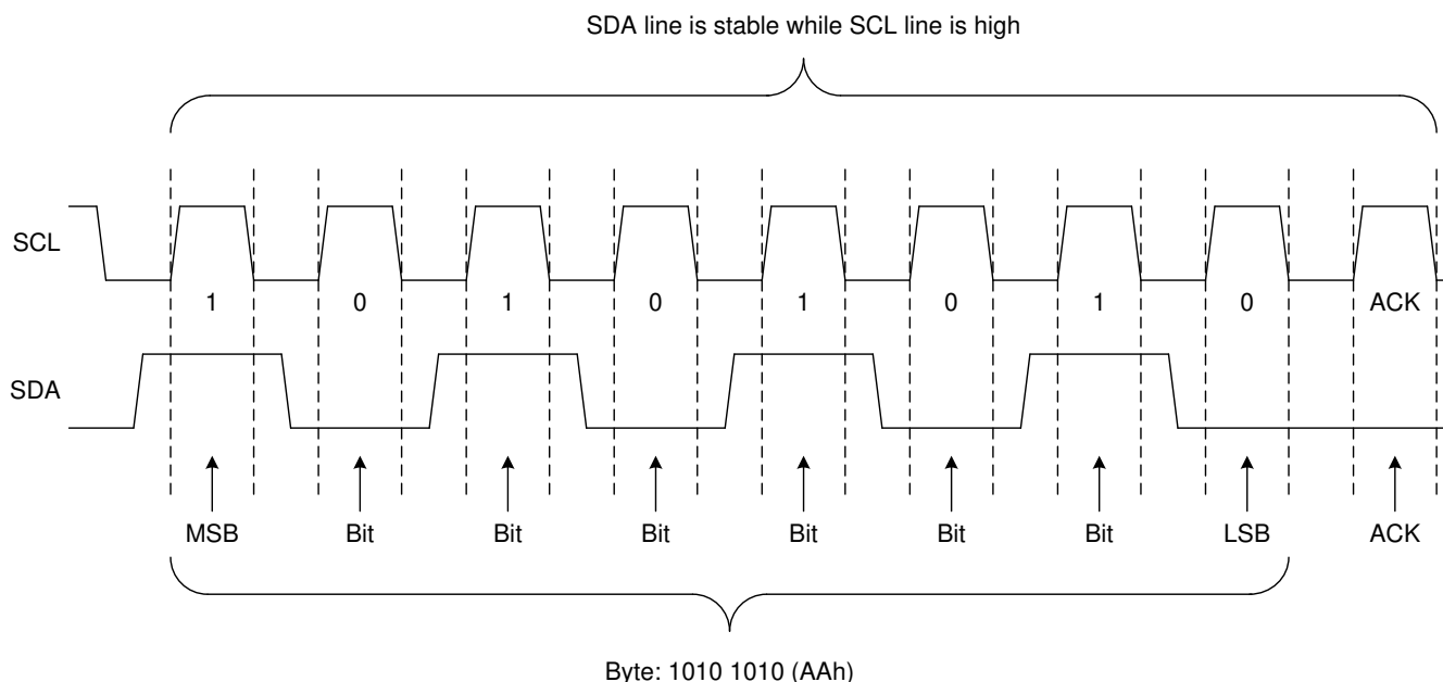
Figure 7-8. Bit Transfer
