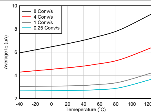
Figure 6-18. Average Supply Current vs Conversion Rate
