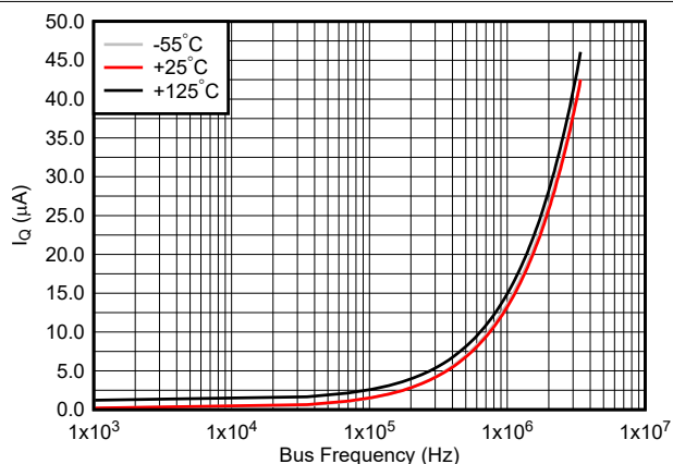
Figure 6-7. Quiescent Current vs Bus Frequency (Temperature at 3.3-V Supply)
