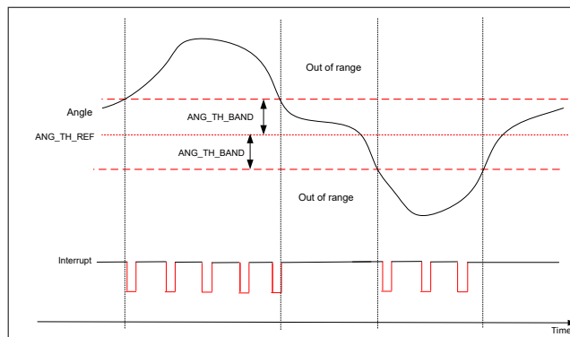
图 7-8. MAG_THR_DIR = 0h、THR_SEL[1:0] = 1h、INT_STATE = 1h 时的角度限值检查
