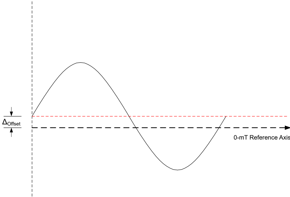
图 7-19. Magnetic Sensor Data Offset Correction
