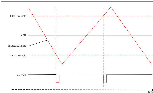
图 8-6. Magnetic Field Going Out of Band Check With MAG_THR_DIR = 0b, THR_HYST = 001b
