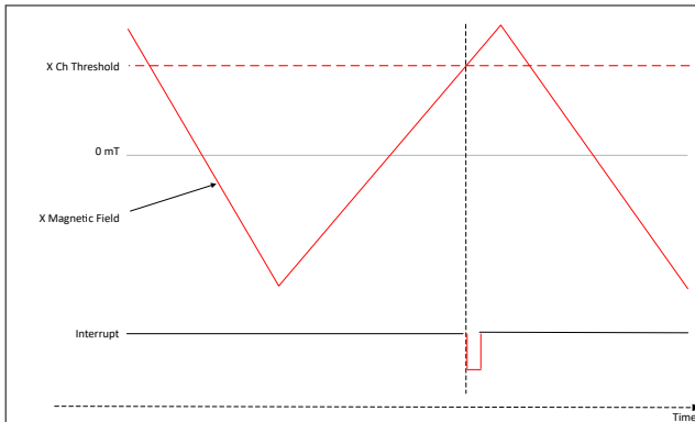
图 8-4. Magnetic Upper Limit Cross Check With MAG_THR_DIR = 0b, THR_HYST = 000b
