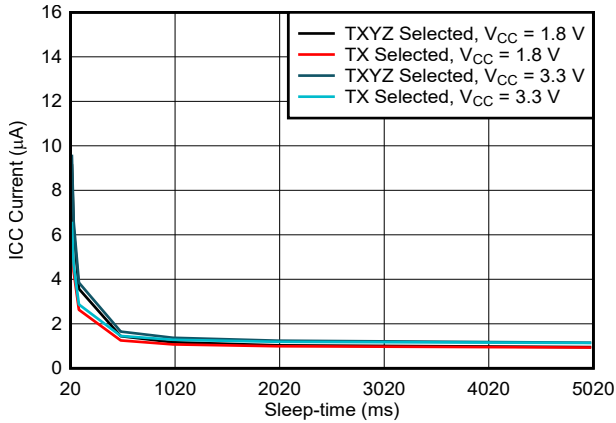
图 6-4. Average ICC vs W&S Mode Sleep Time
