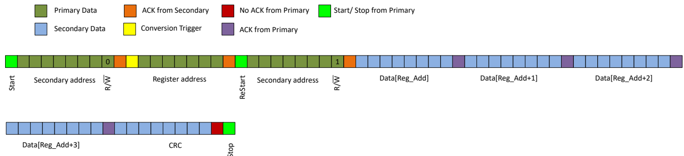
图 7-10. Standard 3-Byte I 2 C Read With CRC Enabled, CRC_EN = 1b
