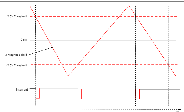
图 8-7. Magnetic Field Entering a Band Check With MAG_THR_DIR = 1b, THR_HYST = 001b
