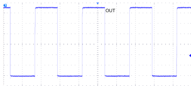
图 9-2. 10-kHz Switching Magnetic Field
