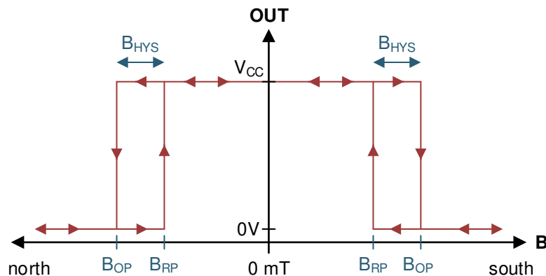
图 6-2. Omnipolar Functionality
