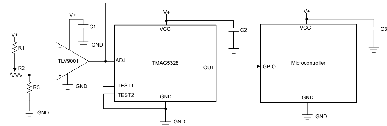
图 7-4. Setting B_{OP} of One TMAG5328 Device Using a Voltage Divider and Potentiometer
