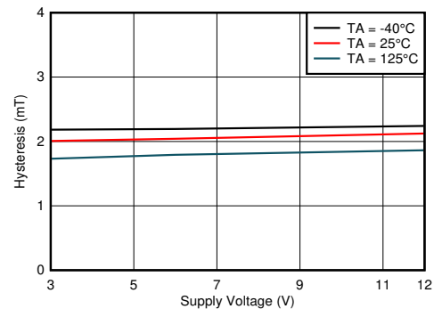
图 7-24. Hysteresis vs. V_{CC}
