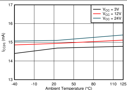
图 7-29. I_{CC(H)} vs. Temperature
