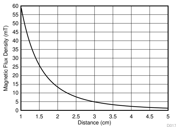
图 9-4. Magnetic Profile of a 1-cm Cube NdFeB Magnet
