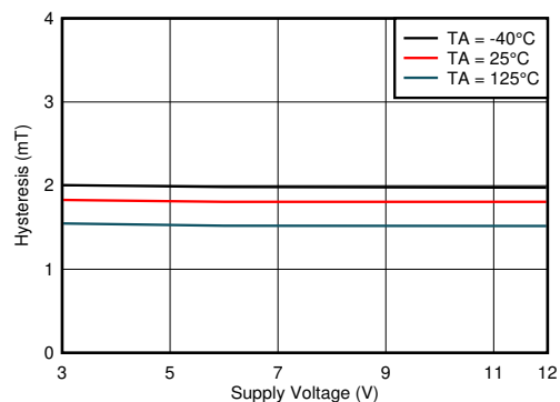
图 7-12. Hysteresis vs. VCC
