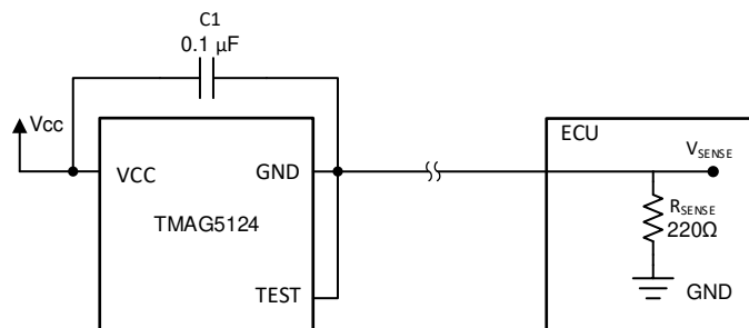
图 9-2. Typical Low-Side Sensing Diagram
