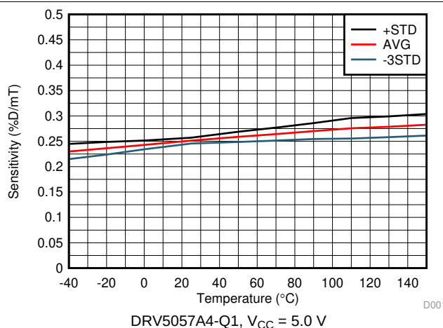
图 10. Sensitivity vs Temperature
