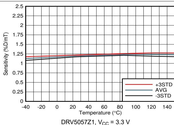
图 6-10. Sensitivity vs Temperature
