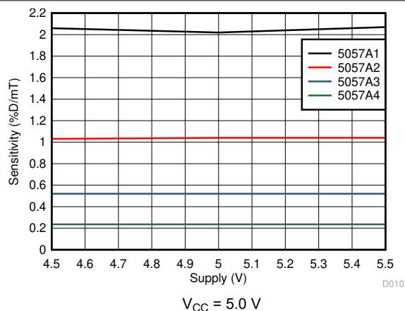
图 6-1. Sensitivity vs Supply Voltage
