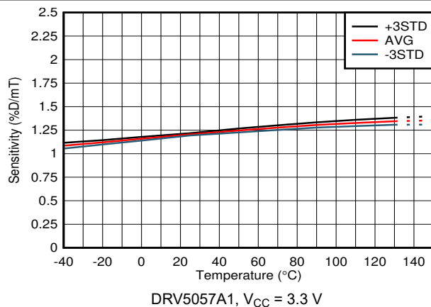
图 6-8. Sensitivity vs Temperature
