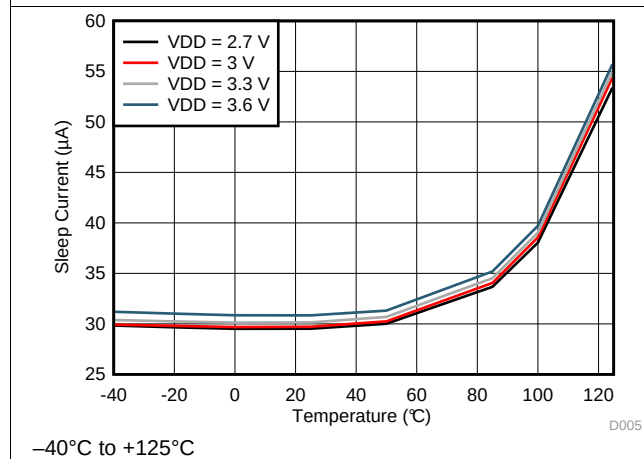
Figure 4. Sleep Mode I_{DD} vs. Temperature
