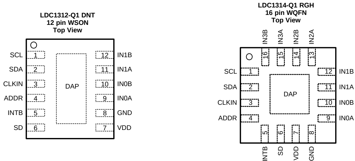
Pin Functions
