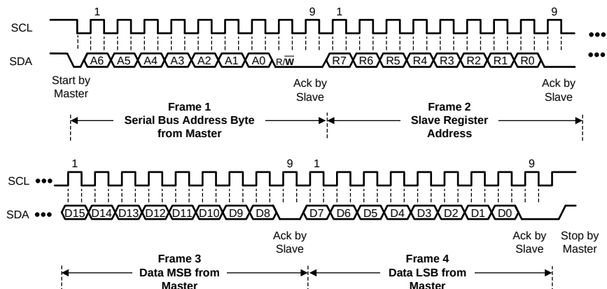
Figure 15. I2C Write Register Sequence
