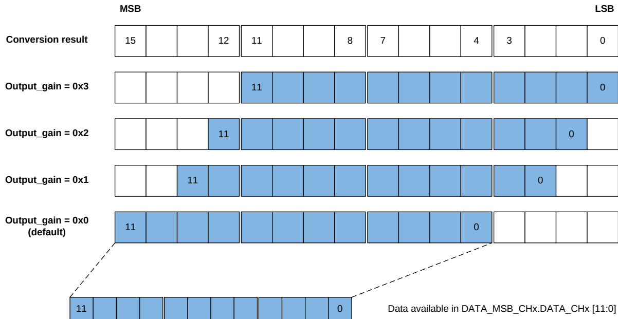
Figure 14. Conversion Data Output Gain
