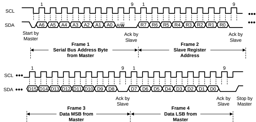
Figure 14. I2C Write Register Sequence
