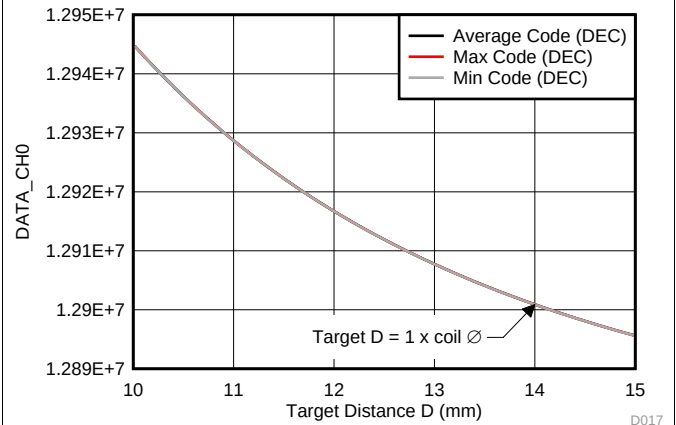
Figure 61. Output Code vs. Target Distance (10 to 15mm)
