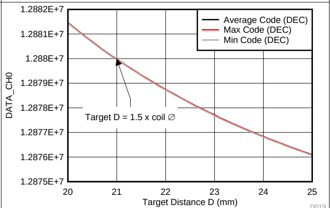
Figure 63. Output Code vs. Target Distance (20 to 25mm)
