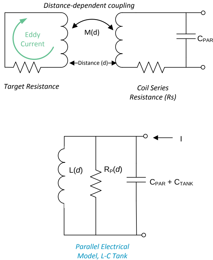
Figure 53. Electrical Model of the L-C Tank Sensor
