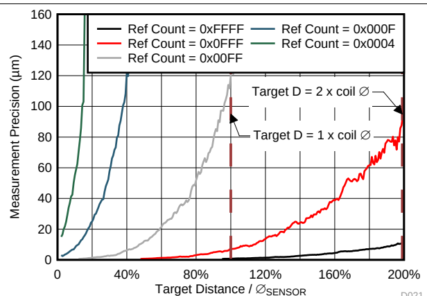
Figure 65. Measurement Precision in Distance vs. Target Distance (0 to 30mm)
