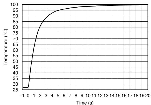
图 8-4. Temperature Step Response
