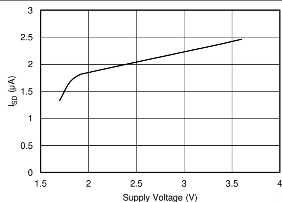
图 6-11. Shutdown Quiescent Current vs. Supply Voltage
