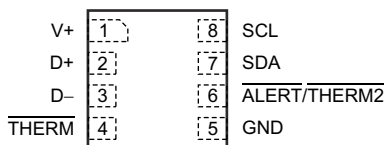
图 5-1. DQF Package 8-Pin WSON Top View
