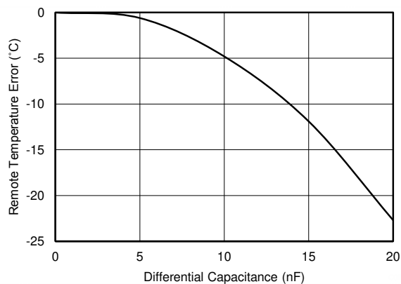
图 6-6. Remote Temperature Error vs. Differential Capacitance
