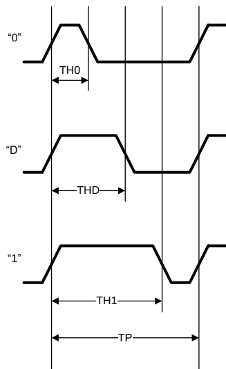
Figure 1. Single-Wire Interface (SWIF) Timing Diagram
