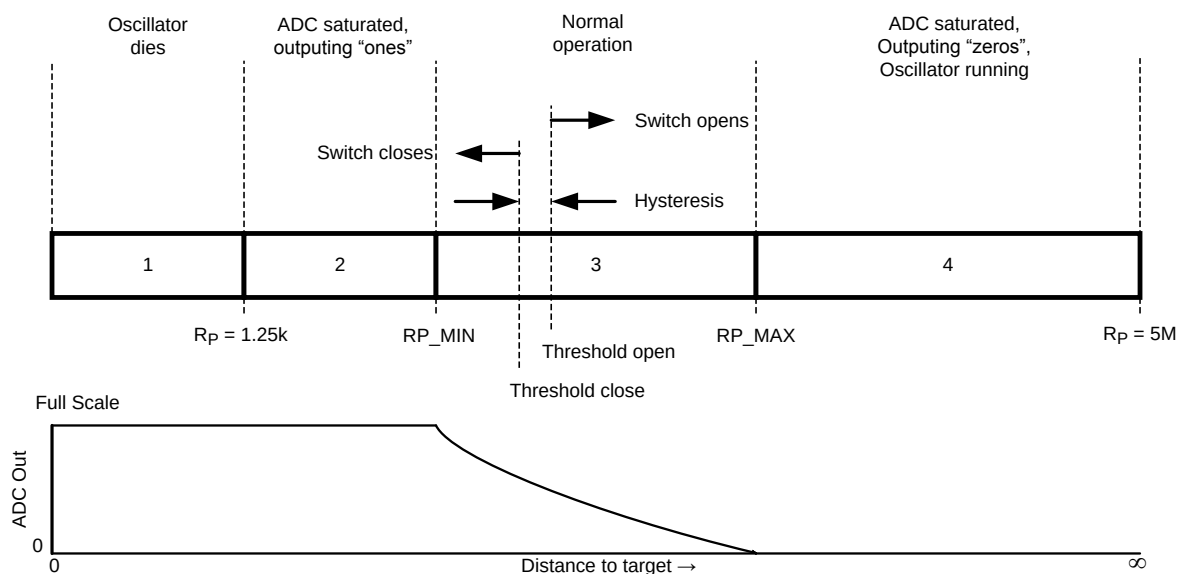
Figure 14. Operating Region
