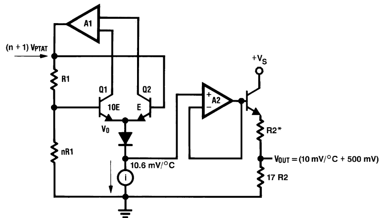
Figure 17. Block Diagram
