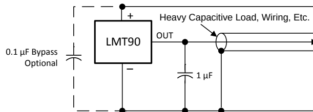
Figure 16. LMT90C with Filter for Noisy Environment
