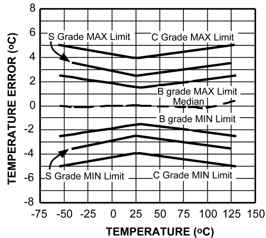
Figure 1. Temperature Error vs Temperature
