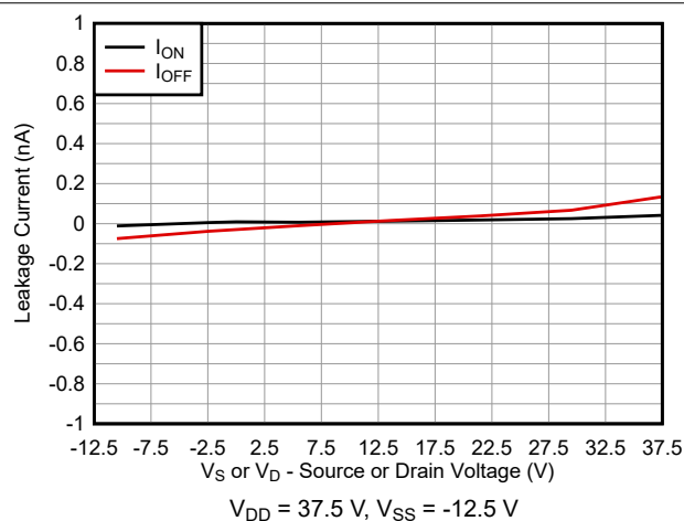
图 6-3. Leakage Current vs Bias Voltage
