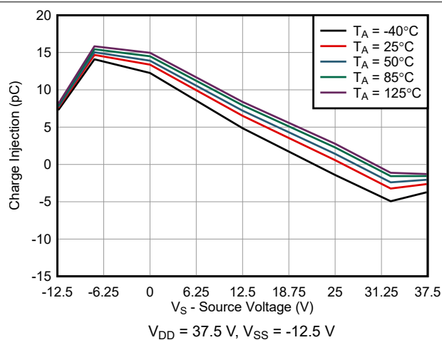
图 6-4. Charge Injection vs Source Voltage
