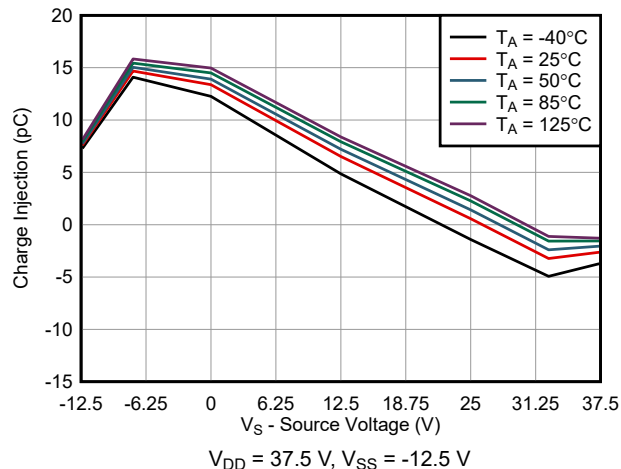
图 8-4. Charge Injection vs Source Voltage
