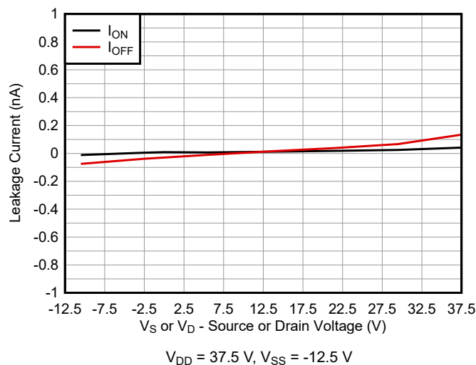
图 7-2. Leakage Current at 50^{\circ}\text{C} vs Bias Voltage
