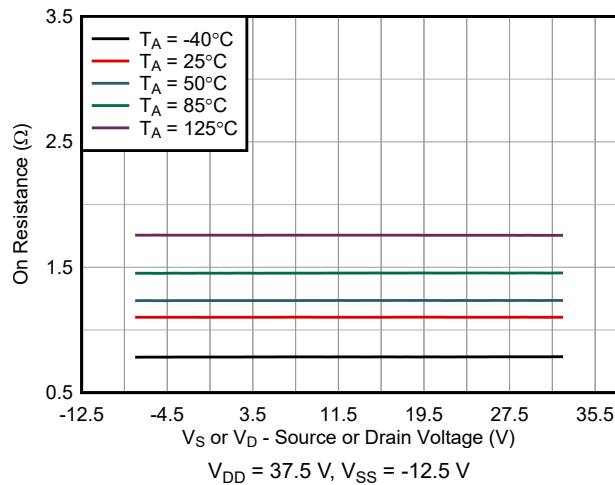
图 8-2. On-Resistance vs Source or Drain Voltage
