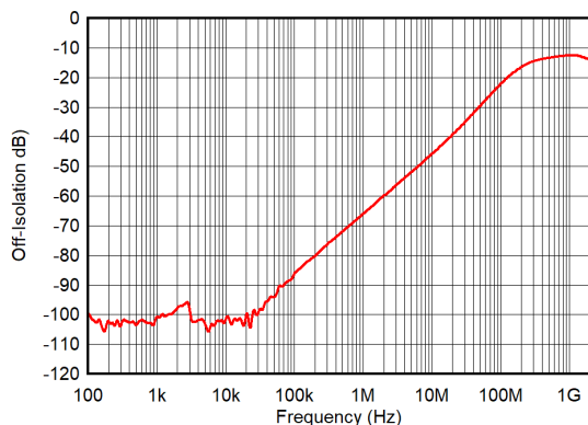
图 6-15. Off-Isolation vs Frequency
