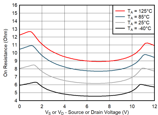
图 6-5. On-Resistance vs Temperature
