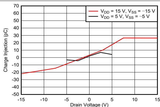
图 6-11. Charge Injection vs Source Voltage - Dual Supply
