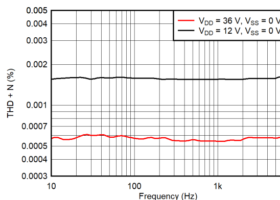
图 6-18. THD+N vs Frequency (Single Supply)
