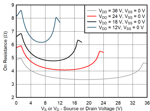
图 6-2. On-Resistance vs Source or Drain Voltage - Single Supply
