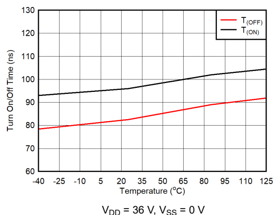
图 6-14. T_{\text{ON}} and T_{\text{OFF}} vs Temperature
