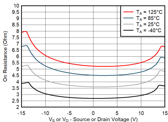
图 6-3. On-Resistance vs Temperature
