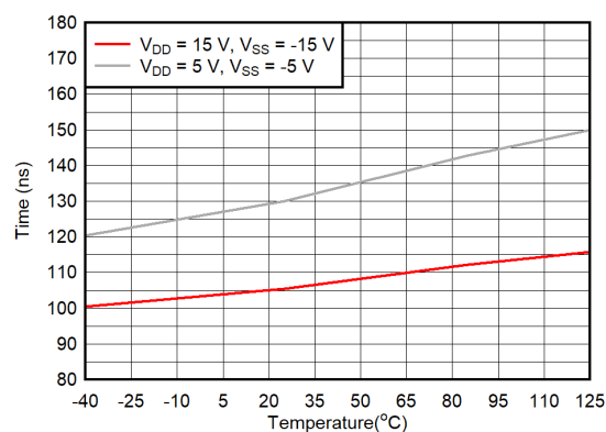
图 6-13. T_{\text{TRANSITION}} vs Temperature
