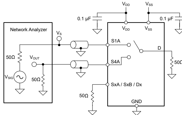
图 7-11. Crosstalk Measurement Setup
