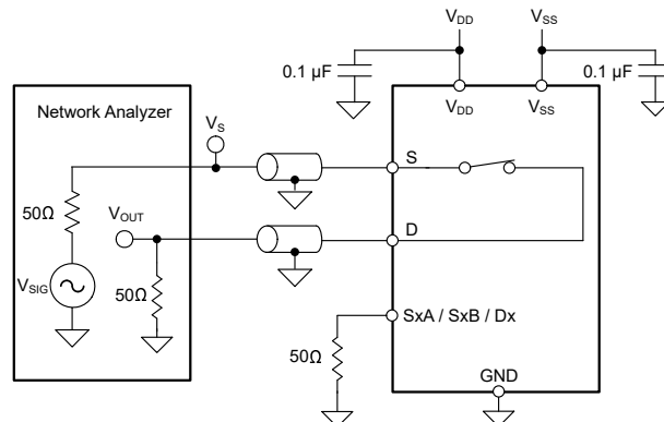
图 7-12. Bandwidth Measurement Setup
