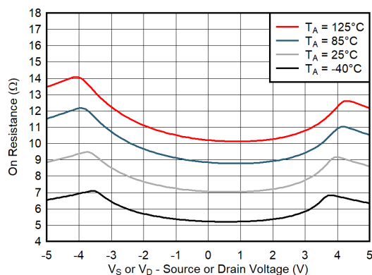
图 6-4. On-Resistance vs Temperature
