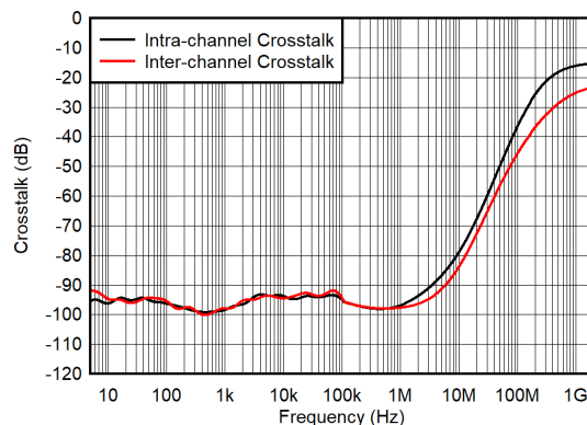
图 6-16. Crosstalk vs Frequency
