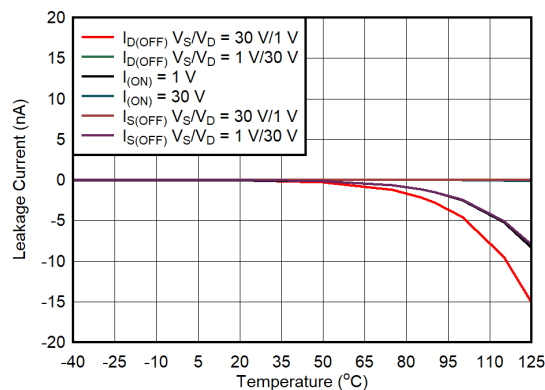
图 6-8. Leakage Current vs Temperature
