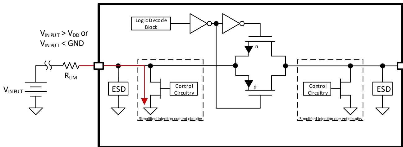
图 9-5. Over-Voltage Event with Series Resistor
