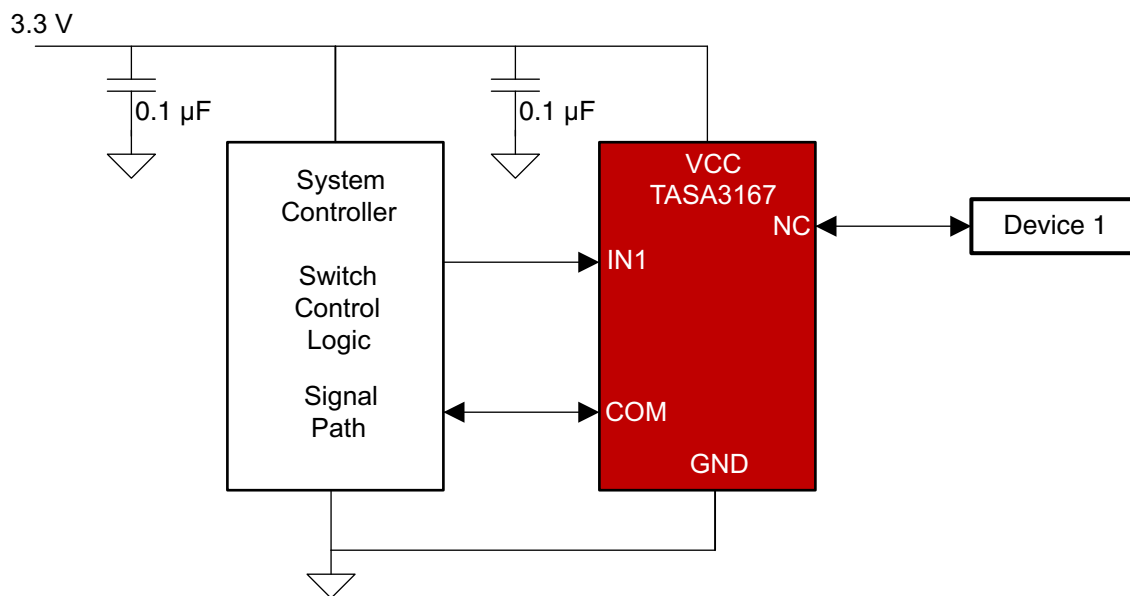
Figure 22. Typical Application
