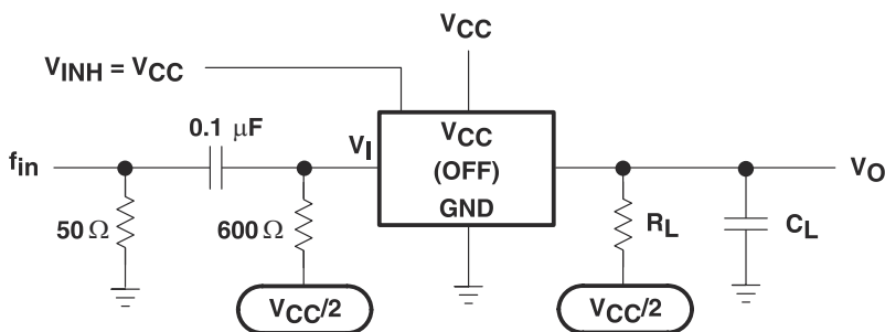
图 6-8. Feedthrough Attenuation (Switch Off)
