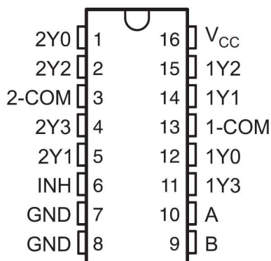
图 4-1. PW Package, 16-Pin TSSOP (Top View)
