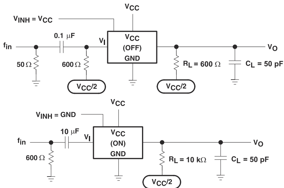
图 6-9. Feedthrough Attenuation (Switch Off)
