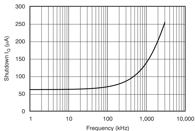
图 7-19. Shutdown I_Q vs I²C Clock Frequency
