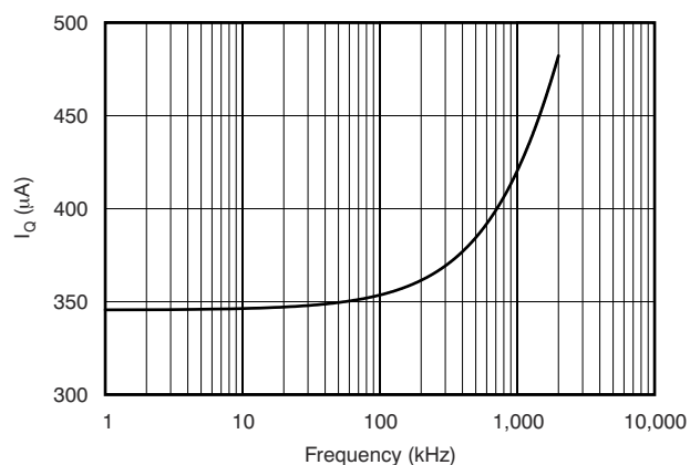
图 7-18. Active I_Q vs I²C Clock Frequency
