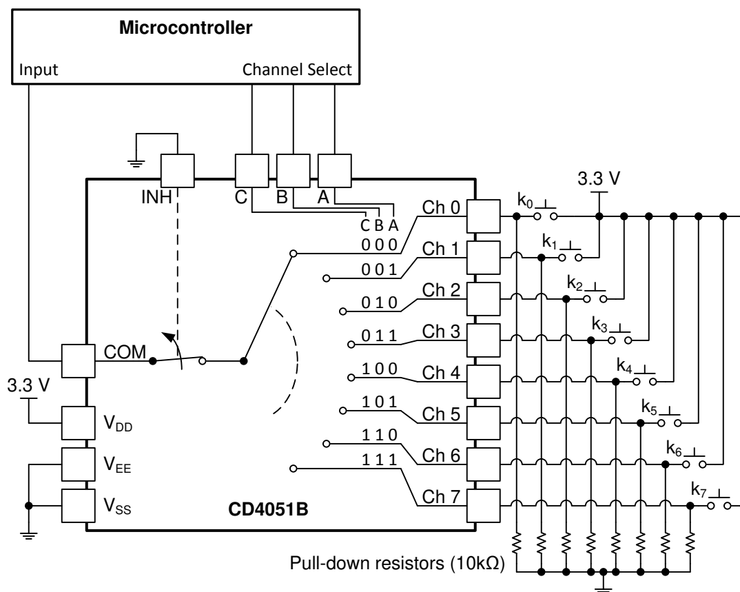
图 9-1. The CD4051B Being Used to Help Read Button Presses on a Keypad
