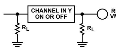
图 7-15. Crosstalk Between Duals or Triplets (CD4052B, CD4053B)
