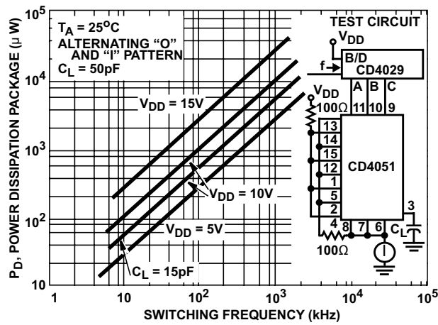
图 6-1. Dynamic Power Dissipation vs Switching Frequency (CD4051B)
