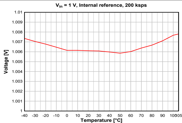
图 7-23. ADC Accuracy vs. Temperature
