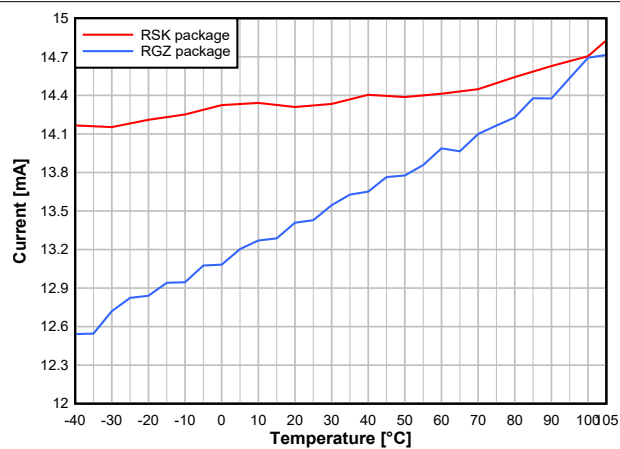
图 7-8. TX Current vs. Temperature (50kbps, 868.3MHz, +10dBm, VDD5 = 3.6V)
