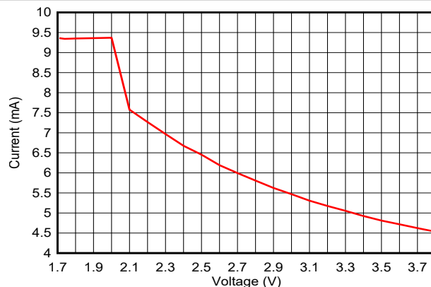
Figure 7-9. RX Current vs. Supply Voltage (VDDS) (BLE 1Mbps, 2.44GHz)
