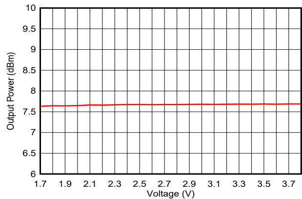
Figure 7-24. Output Power vs. Supply Voltage (VDD) (BLE 1Mbps, 2.44GHz, +8dBm)
