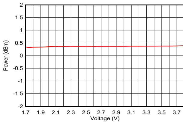
Figure 7-23. Output Power vs. Supply Voltage (VDD) (BLE 1Mbps, 2.44GHz, 0dBm)
