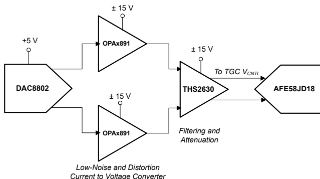
Ultrasound Time-Gain-Control Circuit
