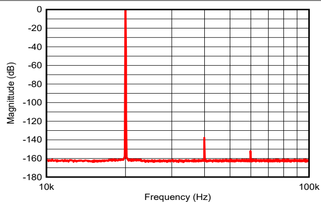
Figure 5-44. 20kHz Output Spectrum
