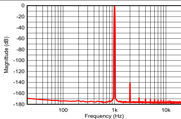
Figure 5-43. 1kHz Output Spectrum
