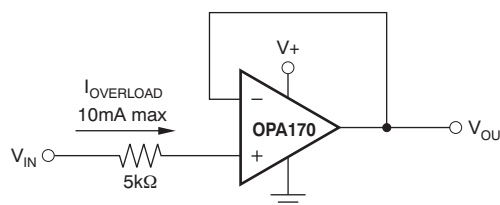
Figure 41. Input Current Protection
