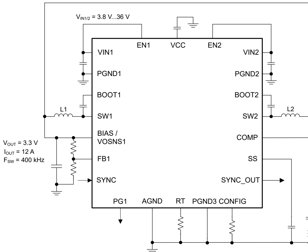
图 9-1. Example Application Circuit - 400-kHz Single Adjustable Output
