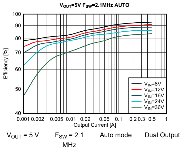
图 9-21. Efficiency
