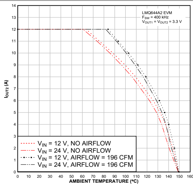
图 9-7. Typical Output Current versus Ambient Temperature, F_{SW} = 400\text{ kHz} , Single Output
