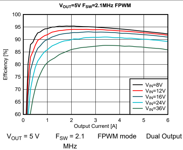
图 9-23. Efficiency
