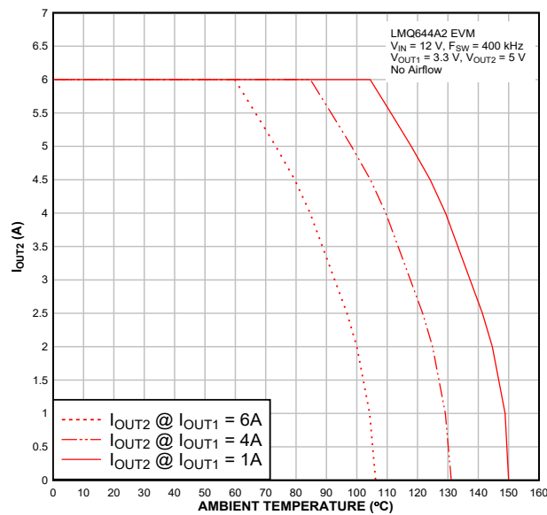
图 9-3. Typical Output Current versus Ambient Temperature, V_{IN} = 12\text{ V} , F_{SW} = 400\text{ kHz} , Dual Output
