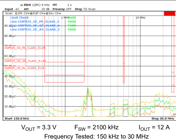
图 9-67. Dual Output Conducted Emissions versus CISPR25 Class 5 Limits (Orange: Peak Signal, Red: Average Signal, Green: Quasi-Peak Signal)
