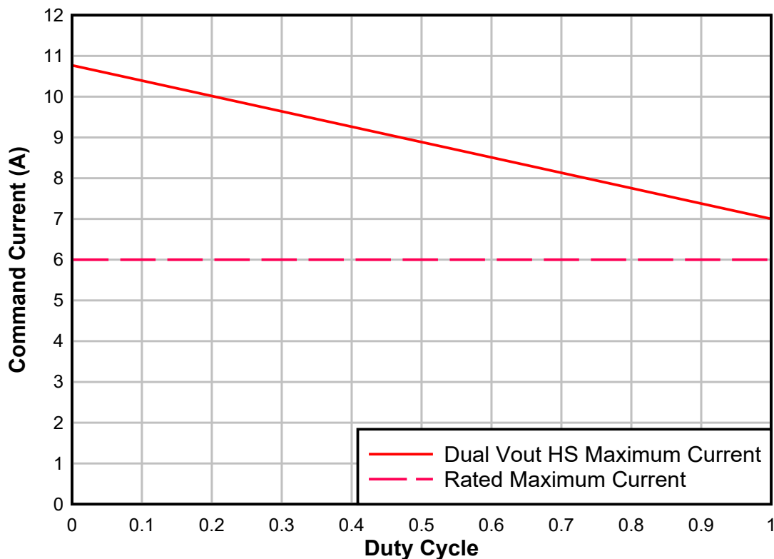
图 8-12. Maximum Current Allowed Through the HS FET - Function of Duty Cycle for LMQ644xx
