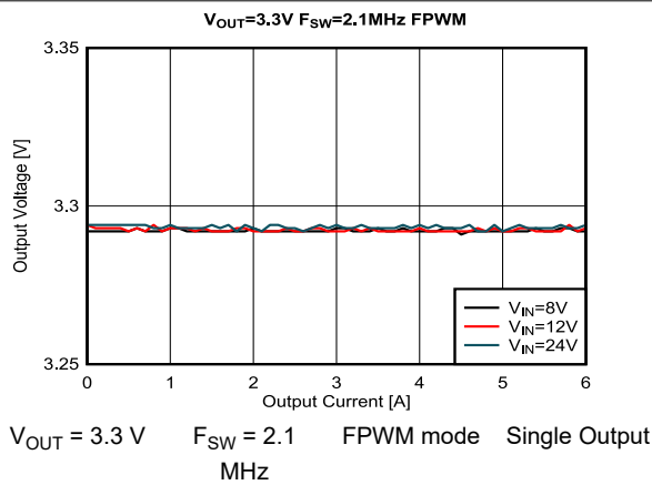
图 9-27. Load and Line Regulation
