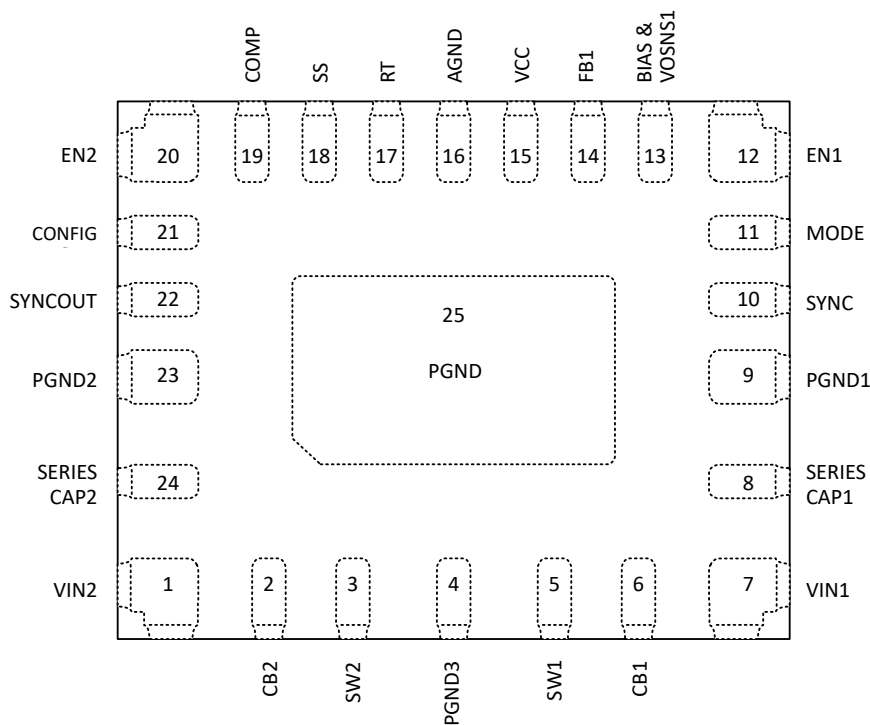
图 6-3. Single Output Secondary (Top View)
