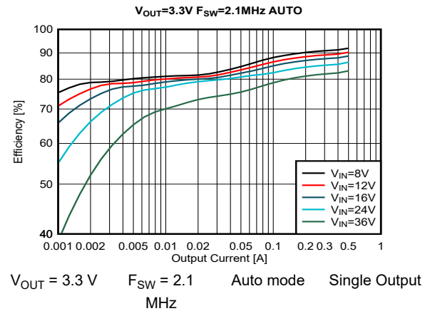
图 9-18. Efficiency
