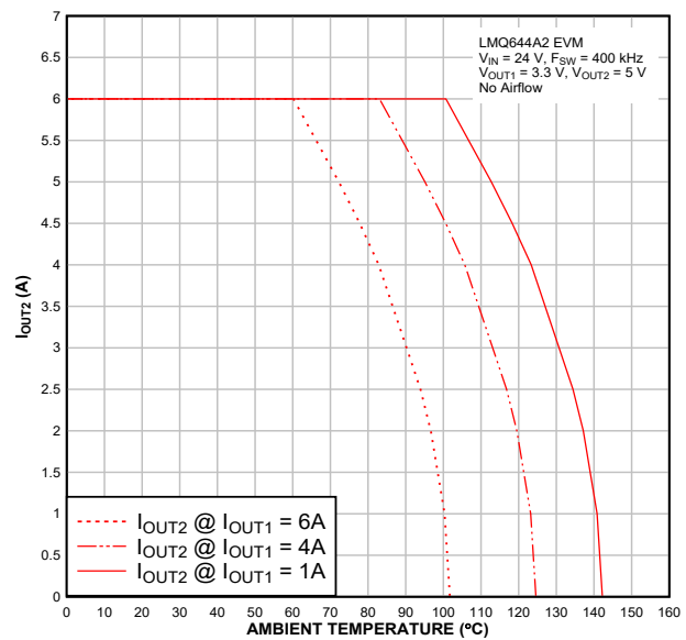
图 9-4. Typical Output Current versus Ambient Temperature, V_{IN} = 24\text{ V} , F_{SW} = 400\text{ kHz} , Dual Output
