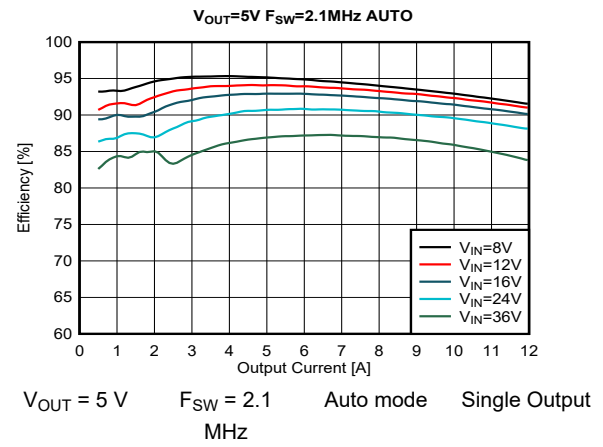
图 9-16. Efficiency
