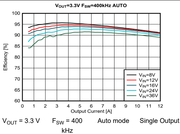
图 9-13. Efficiency
