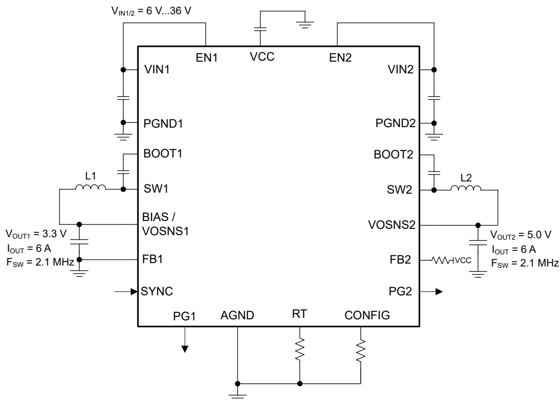
图 9-2. Example Application Circuit - 2.1-MHz Dual Fixed Output
