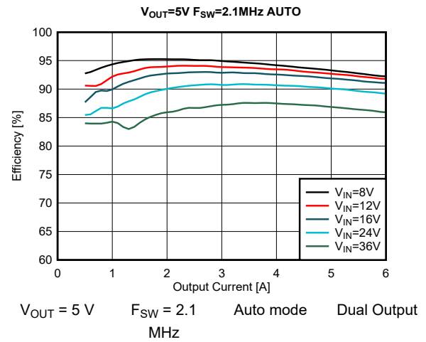
图 9-22. Efficiency
