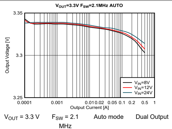
图 9-30. Load and Line Regulation
