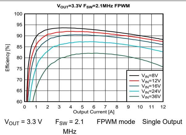
图 9-20. Efficiency
