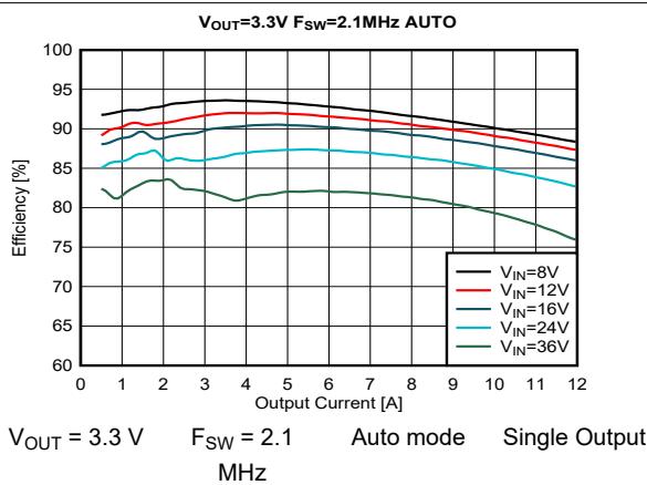
图 9-19. Efficiency
