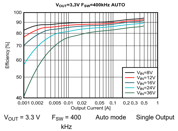
图 9-12. Efficiency
