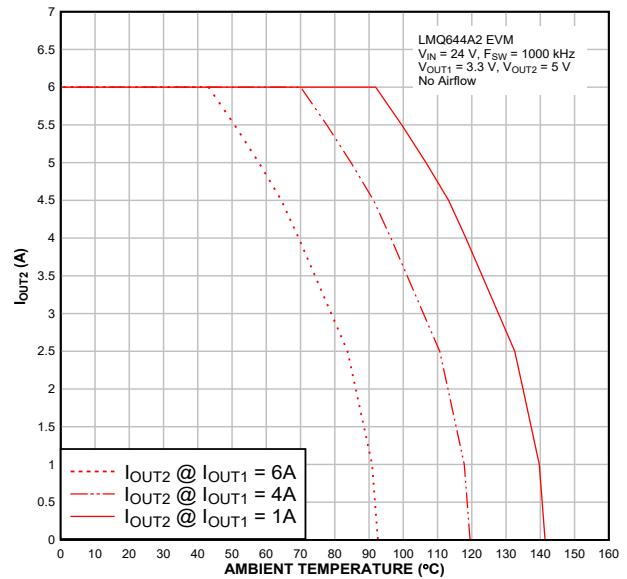
图 9-6. Typical Output Current versus Ambient Temperature, V_{IN} = 24\text{ V} F_{SW} = 1\text{ MHz} , Dual Output
