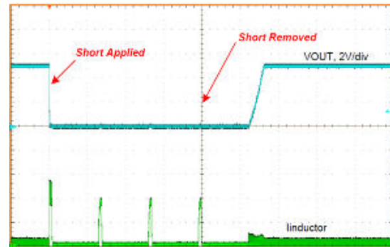
图 8-15. Short-Circuit Transient and Recovery
