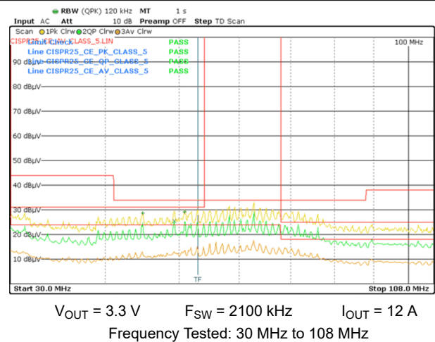
图 9-68. Dual Output Conducted Emissions versus CISPR25 Class 5 Limits (Orange: Peak Signal, Red: Average Signal, Green: Quasi-Peak Signal)
