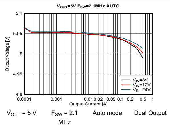
图 9-32. Load and Line Regulation
