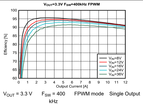
图 9-14. Efficiency
