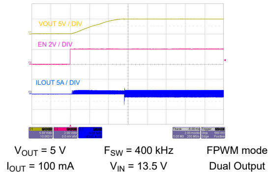
图 9-38. Start-Up With 100-mA Load
