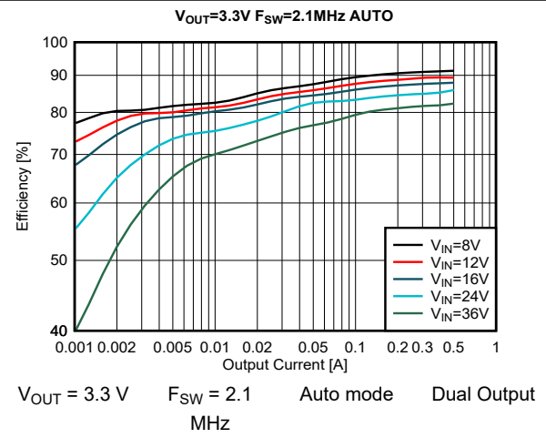
图 9-24. Efficiency
