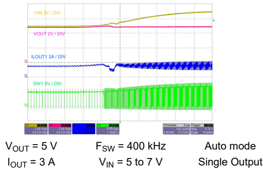
图 9-37. Dropout Recovery
