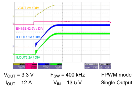
图 9-40. Start-Up With 12-A Load
