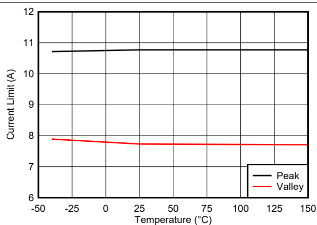
图 7-4. High-side and Low-side Current Limits LMQ644A2
