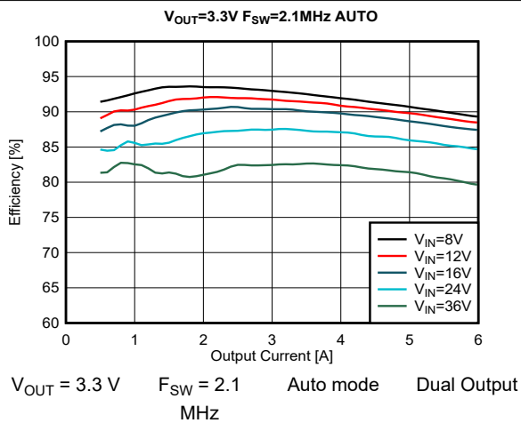
图 9-25. Efficiency
