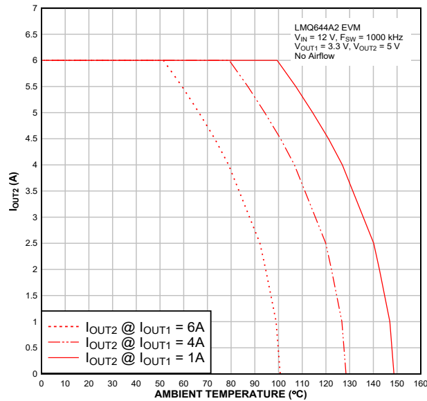
图 9-5. Typical Output Current versus Ambient Temperature, V_{IN} = 12\text{ V} F_{SW} = 1\text{ MHz} , Dual Output
