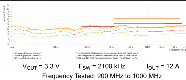
图 9-65. Dual Output Log Radiated Emissions versus CISPR25 Class 5 Limits (Orange: Peak Signal, Red: Average Signal, Green: Quasi-Peak Signal)
