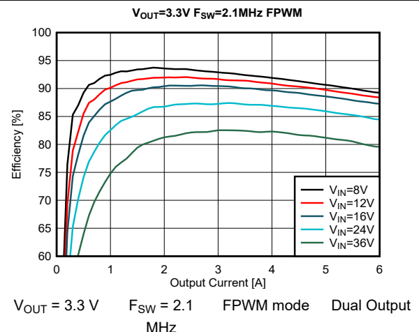
图 9-26. Efficiency
