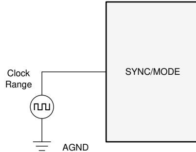
图 8-4. Typical Implementation Allowing Synchronization Using the SYNC/MODE Pin
