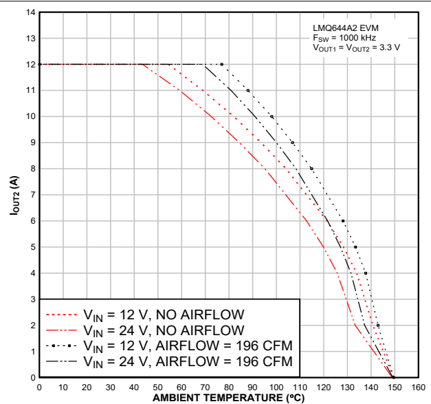
图 9-8. Typical Output Current versus Ambient Temperature, F_{SW} = 1\text{ MHz} , Single Output
