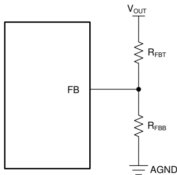
图 8-3. Setting Output Voltage of Adjustable Versions
