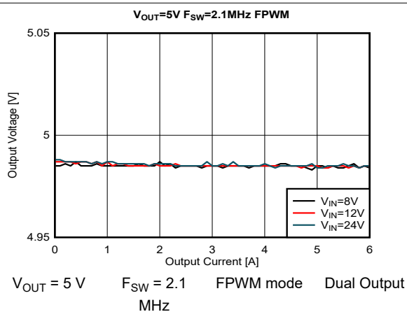
图 9-31. Load and Line Regulation
