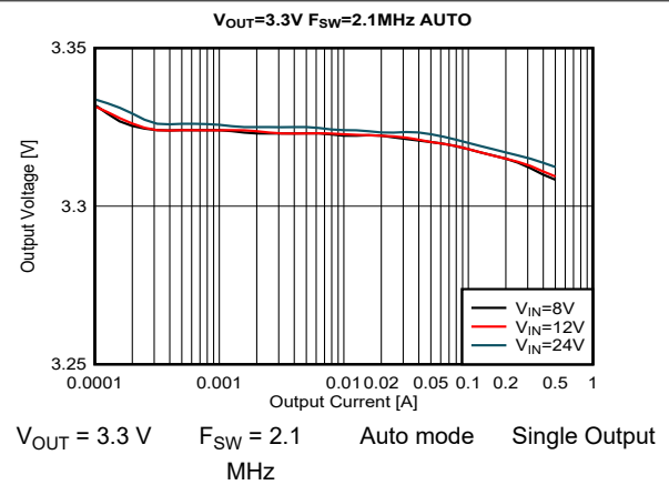
图 9-28. Load and Line Regulation
