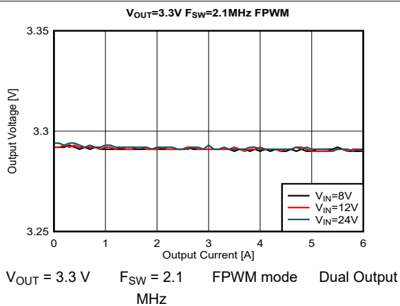
图 9-29. Load and Line Regulation
