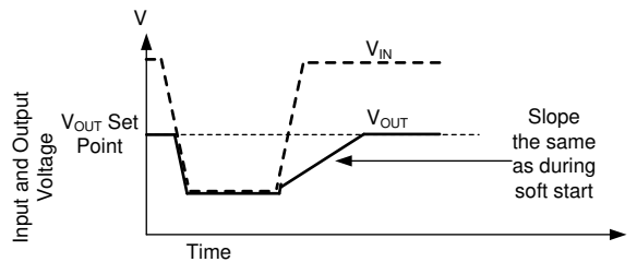
图 8-21. When Output Voltage Falls, It Recovers Slowly Preventing Overshoot and Large Inrush Currents
