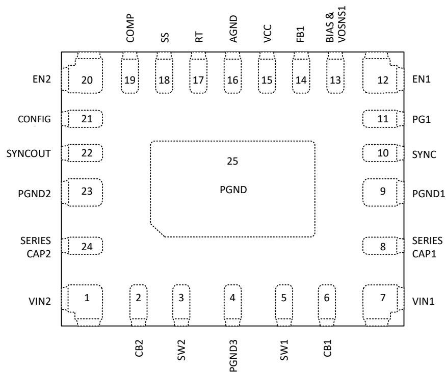
图 6-2. Single Output Primary (Top View)
