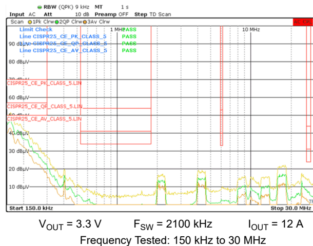
图 9-61. Single Output Conducted Emissions versus CISPR25 Class 5 Limits (Orange: Peak Signal, Red: Average Signal, Green: Quasi-Peak Signal)
