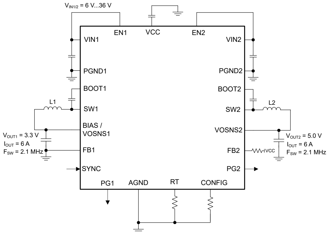
图 8-1. Dual-Output Regulator Schematic Diagram With Input Voltage Operating Range of 6 V to 36 V
