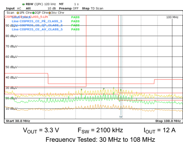
图 9-62. Single Output Conducted Emissions versus CISPR25 Class 5 Limits (Orange: Peak Signal, Red: Average Signal, Green: Quasi-Peak Signal)
