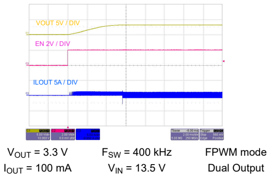
图 9-39. Start-Up With 100-mA Load
