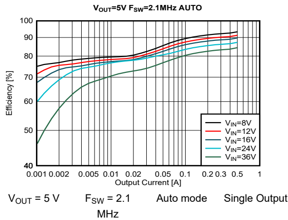
图 9-15. Efficiency
