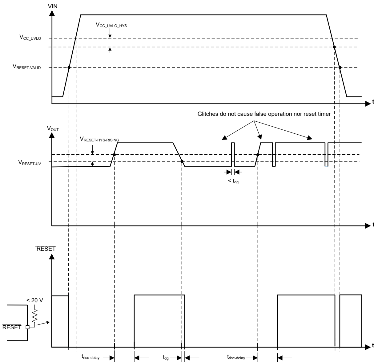
图 8-8. PG Timing Diagram (Excludes OV Events)
