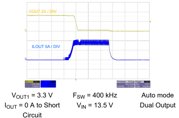
图 9-42. Short-Circuit Protection
