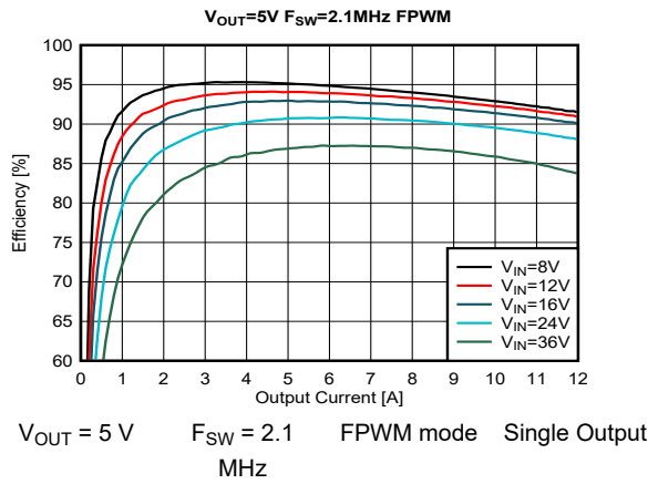
图 9-17. Efficiency
