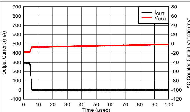
Figure 5-22. Load Transient
