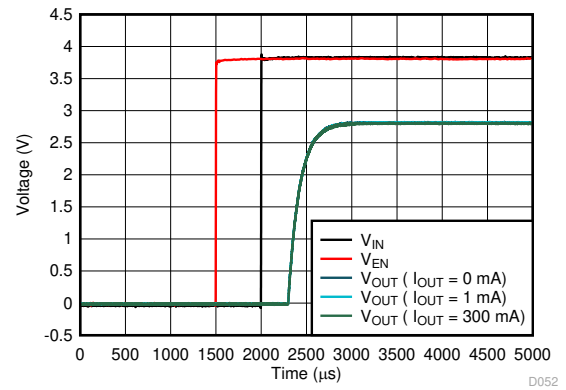
Figure 5-38. Start-Up
