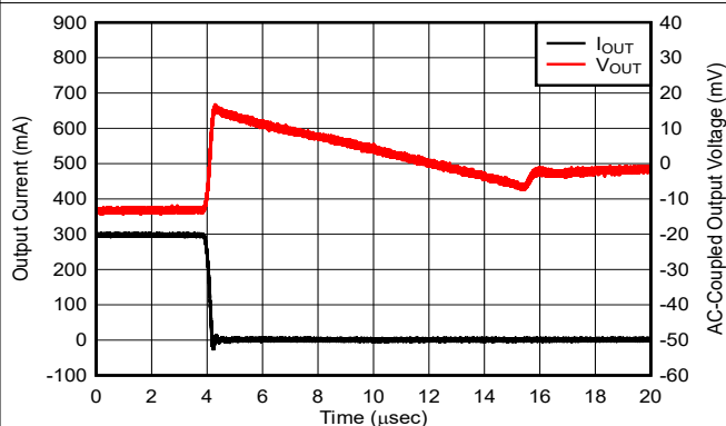
Figure 5-20. Load Transient
