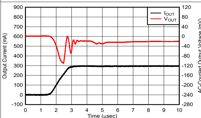
Figure 5-21. Load Transient
