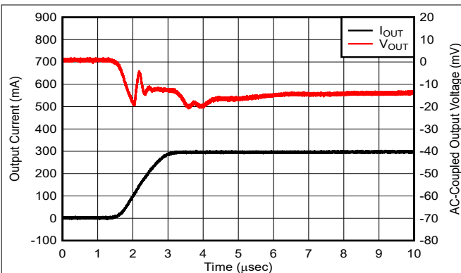
Figure 5-19. Load Transient
