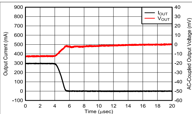
Figure 5-20. Load Transient
