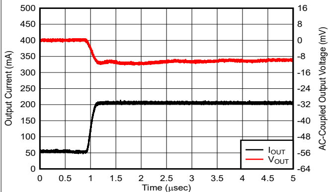
Figure 5-15. Load Transient
