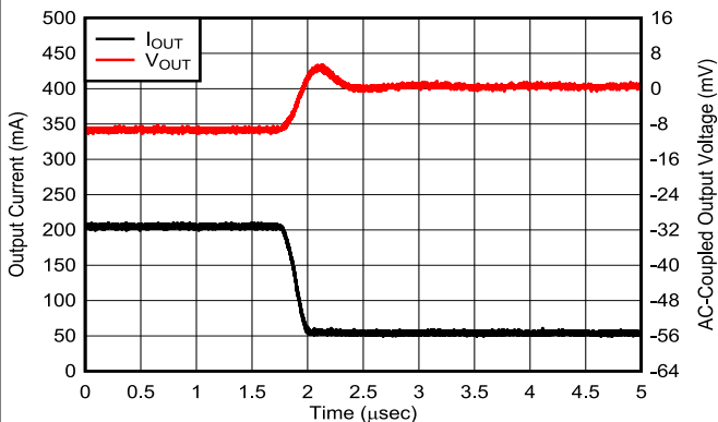
Figure 5-16. Load Transient
