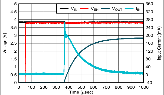
Figure 5-38. Start-Up
