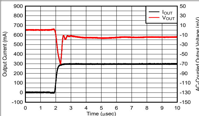
Figure 5-19. Load Transient
