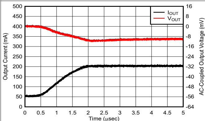
Figure 5-15. Load Transient
