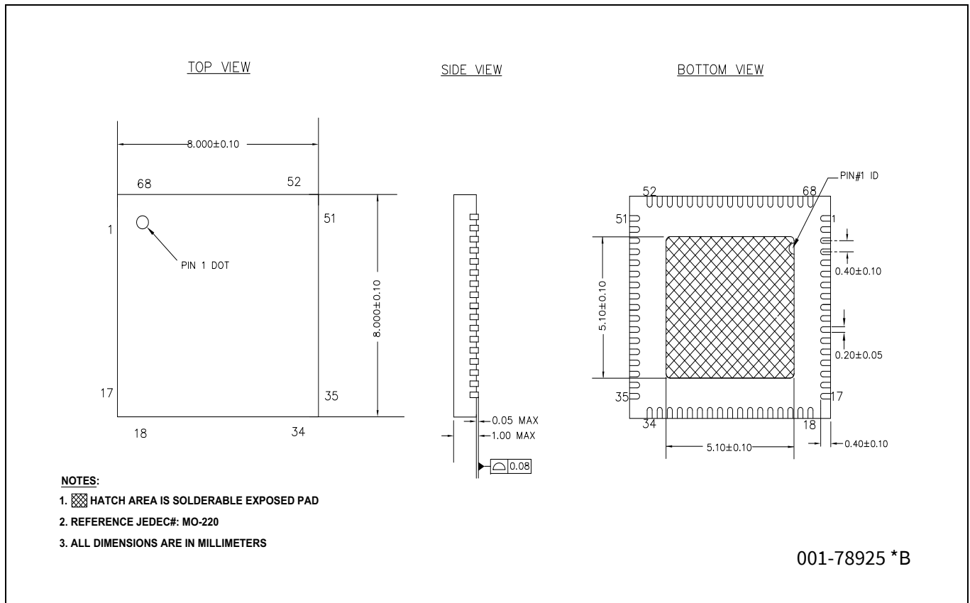
Figure 19 68L QFN (8 × 8 × 1.0 mm) LT68B 5.1 × 5.1 mm EPAD (SAWN), package outline (PG-VQFN-68)
