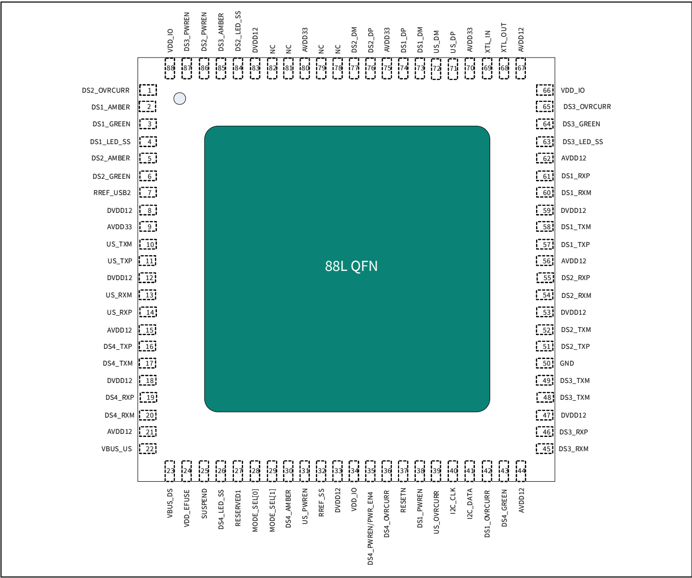
Figure 14 88L QFN pinout for CYUSB3314 and CYUSB2312
