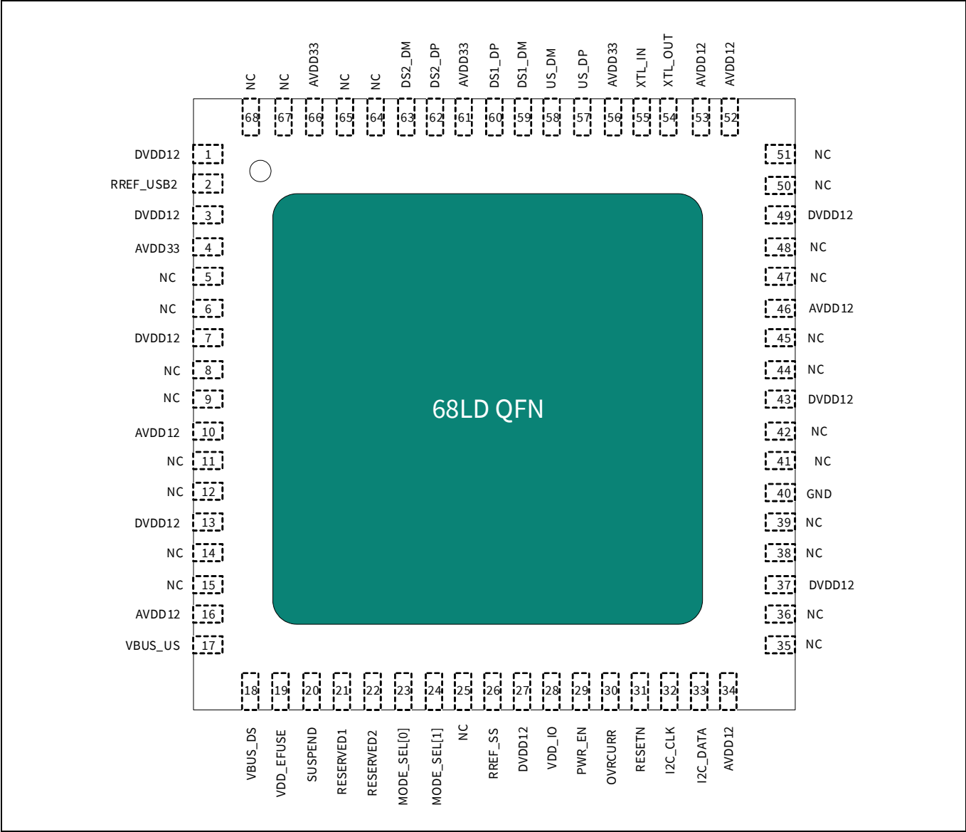
Figure 11 68L QFN pinout for CYUSB2304
