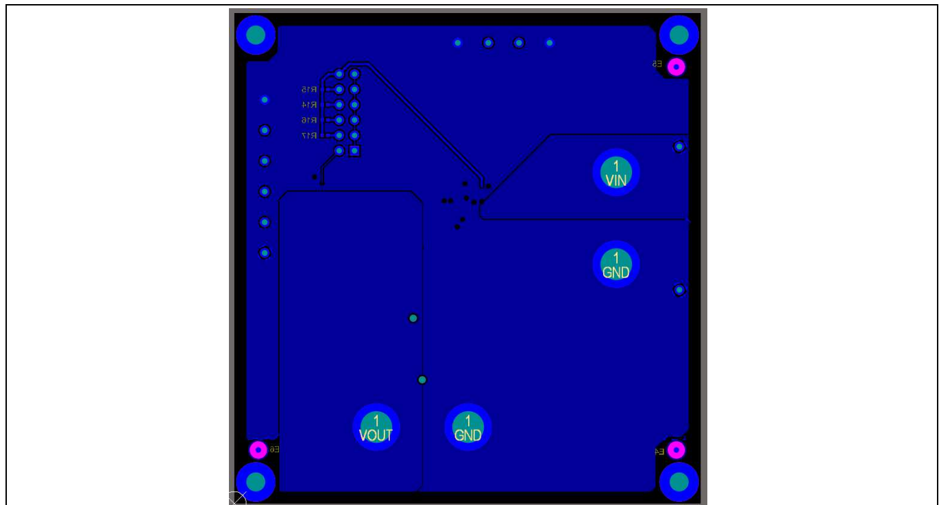
Figure 11 TDA38806 Demo Board – Bottom Layer
