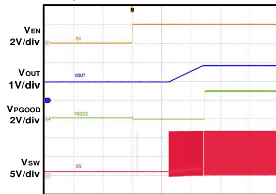
Pre-Bias Start-Up FCCM, No Load
