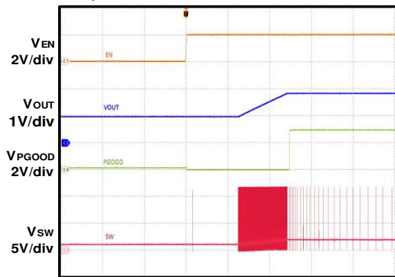
Pre-Bias Start-Up DEM, No Load
