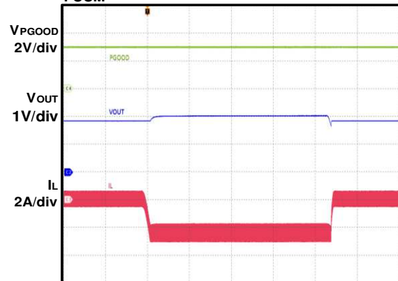
OSM Operation FCCM
