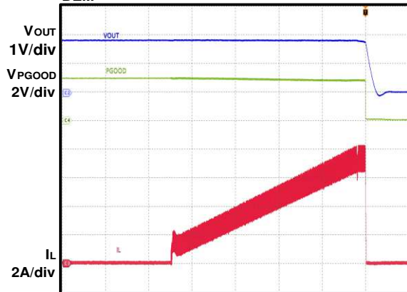
Over-Current Protection DEM
