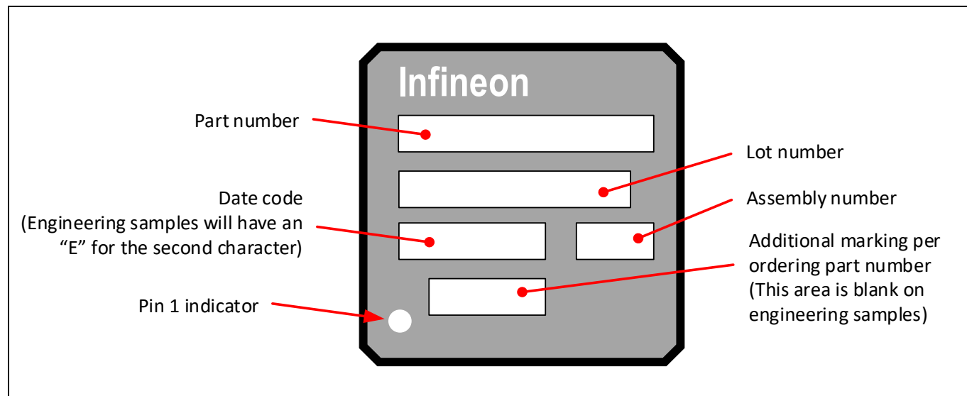
Figure 2 Package marking
