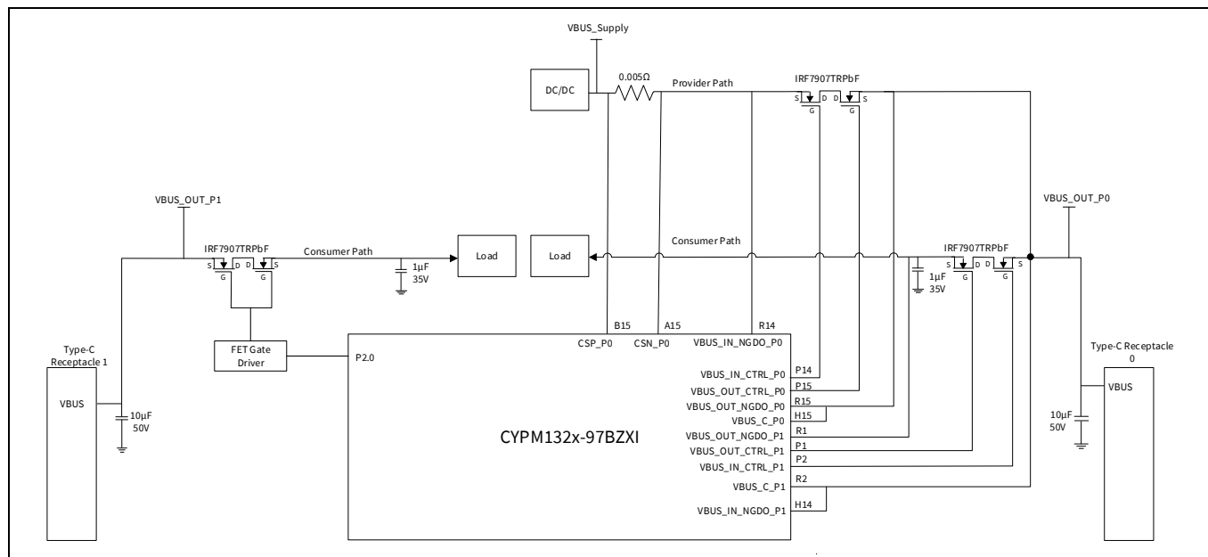
Figure 13 DRP on one Type-C port and sink on the second Type-C port using 97-ball BGA
