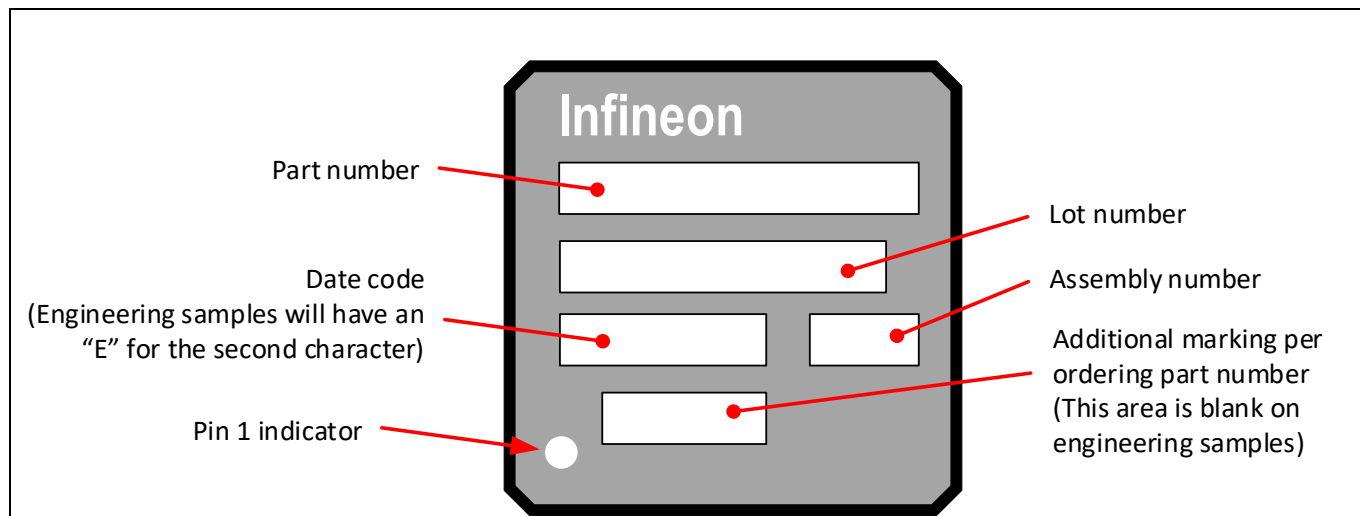
Figure 2 Package marking
