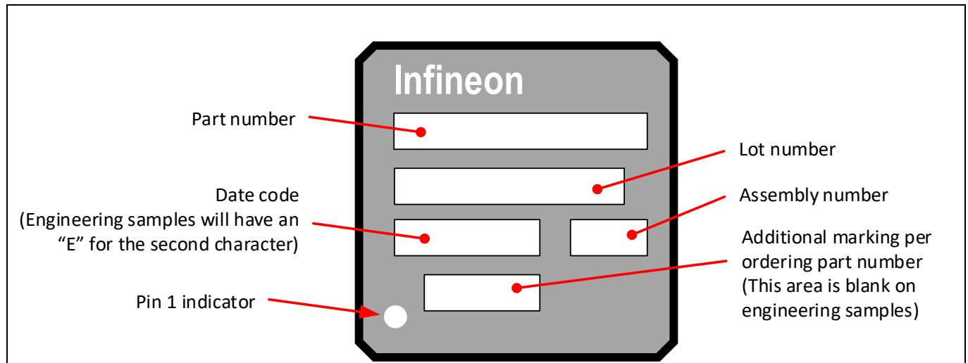
Figure 2 Package marking
