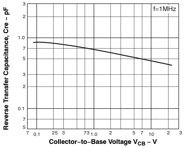
Figure 4. C_{re} - V_{CB}
