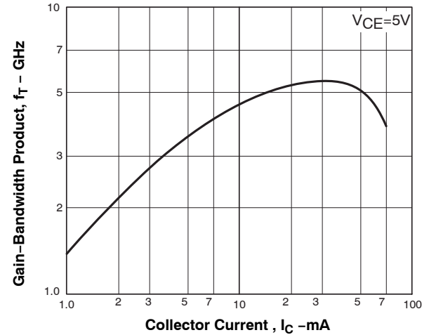
Figure 4. f_T - I_C
