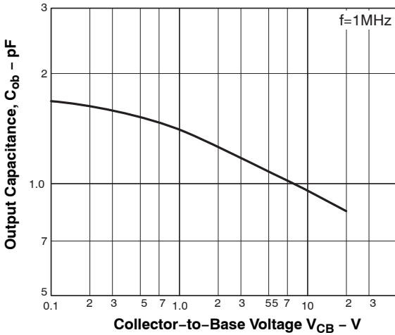
Figure 5. C_{ob} - V_{CB}
