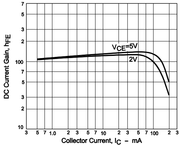
Figure 3. h_{FE} - I_C
