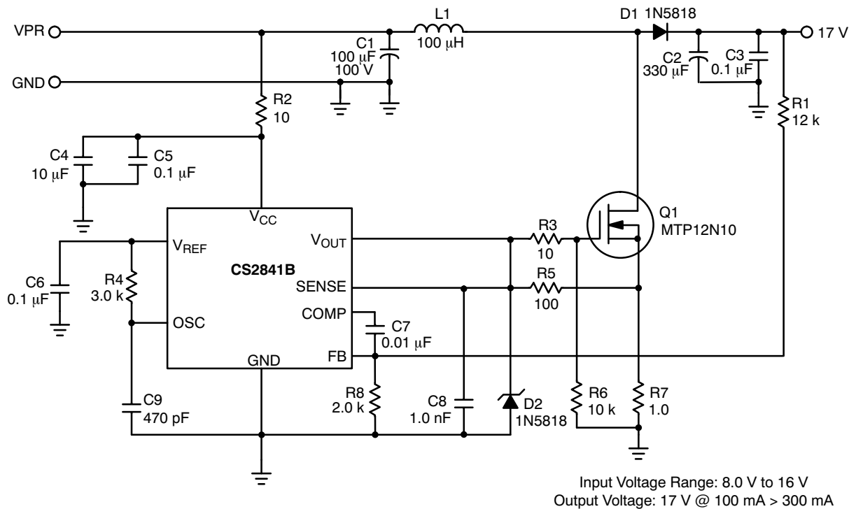
Figure 9. Boost Application
